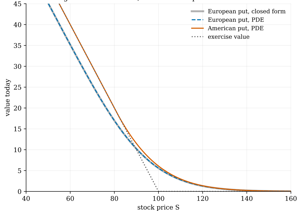
Checked against Black-Scholes; the American premium
