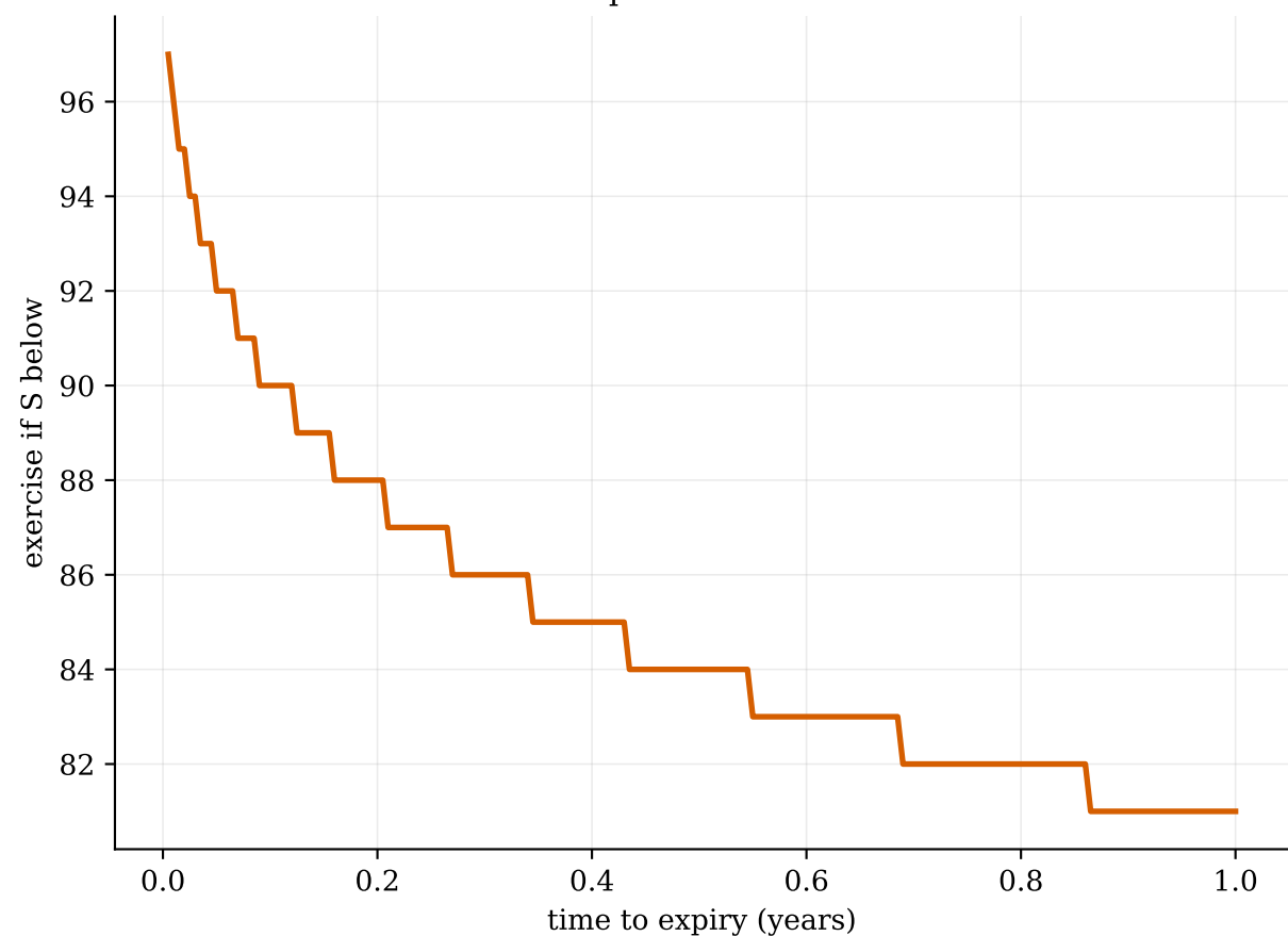
When to exercise an American put
