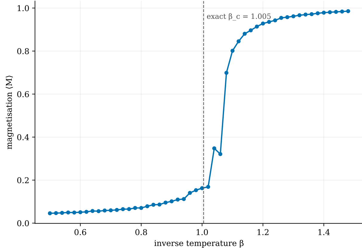
3-state Potts model, 24 \times 24 : order appears
