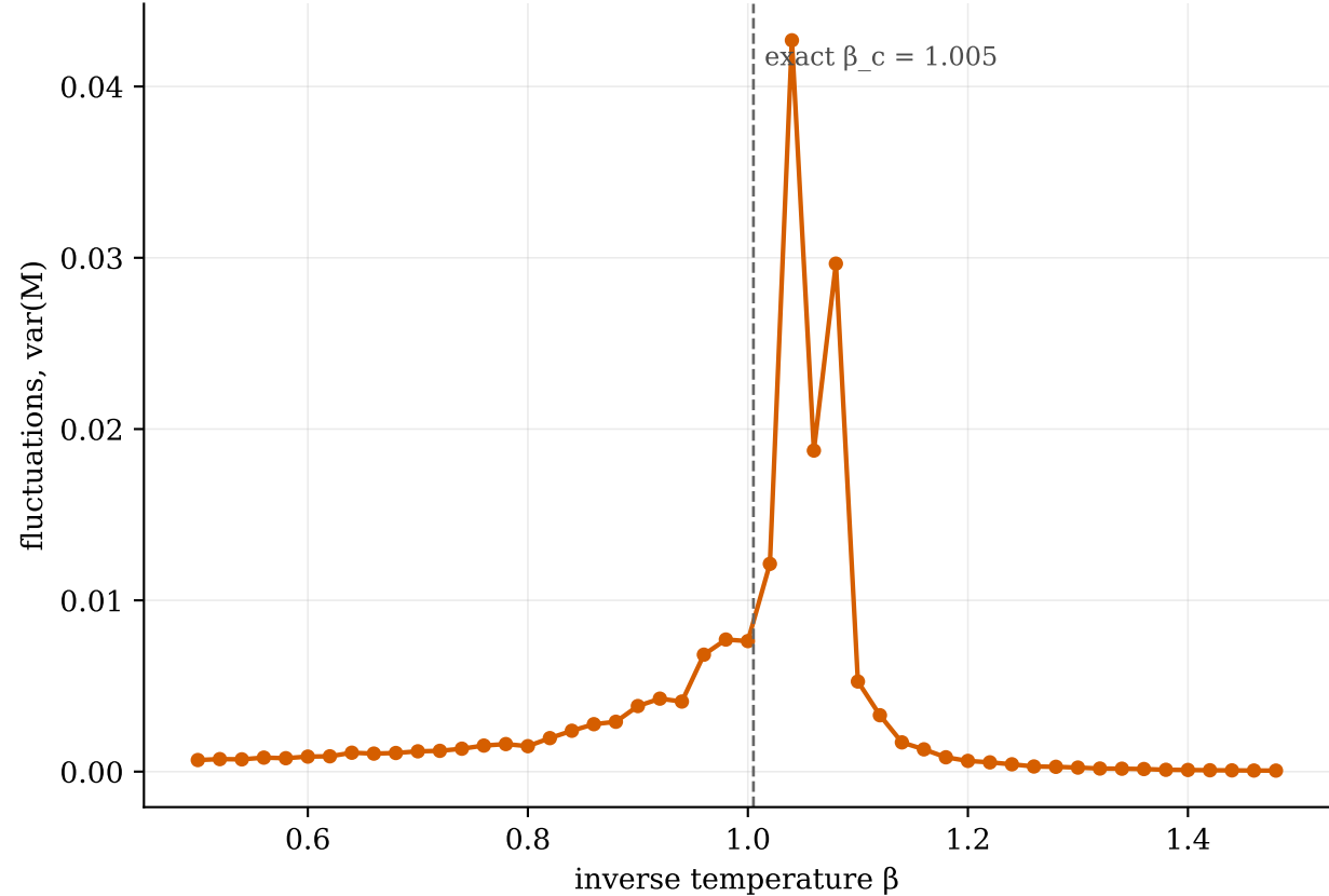
Fluctuations peak at the transition
