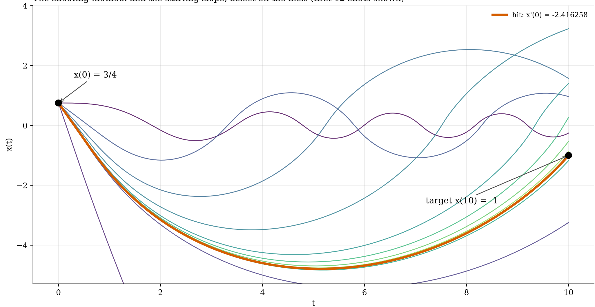
The shooting method: aim the starting slope, bisect on the miss (first 12 shots shown)
