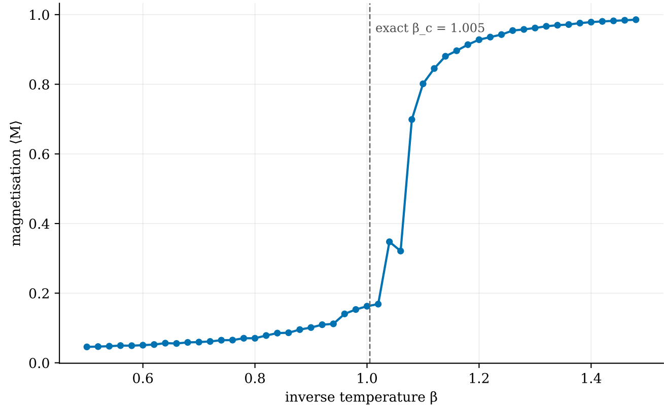
Order appears: magnetisation, 24 \times 24 lattice (C++ output)
