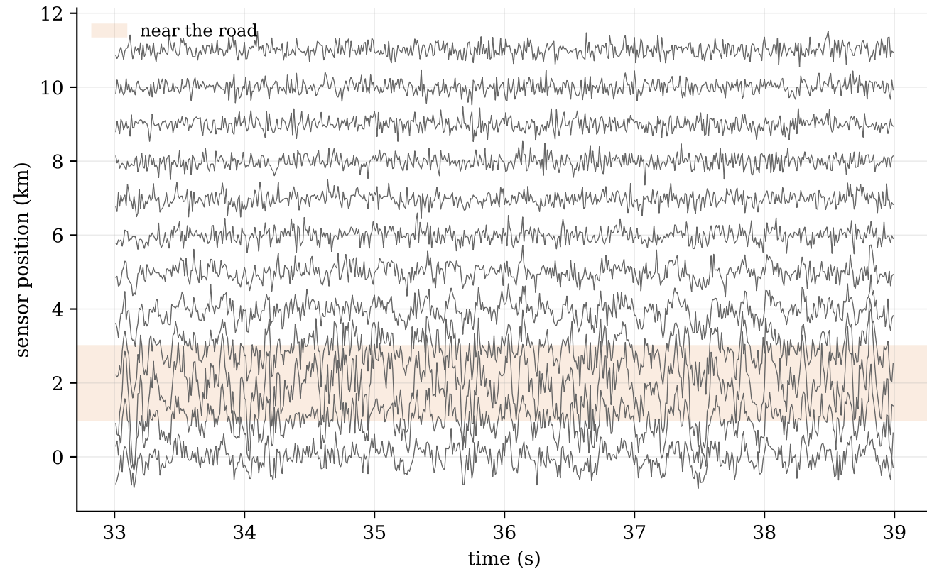
Raw traces: one wave, road noise on some sensors
