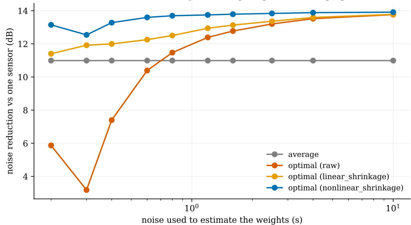
32 sensors: when optimal weighting beats averaging
