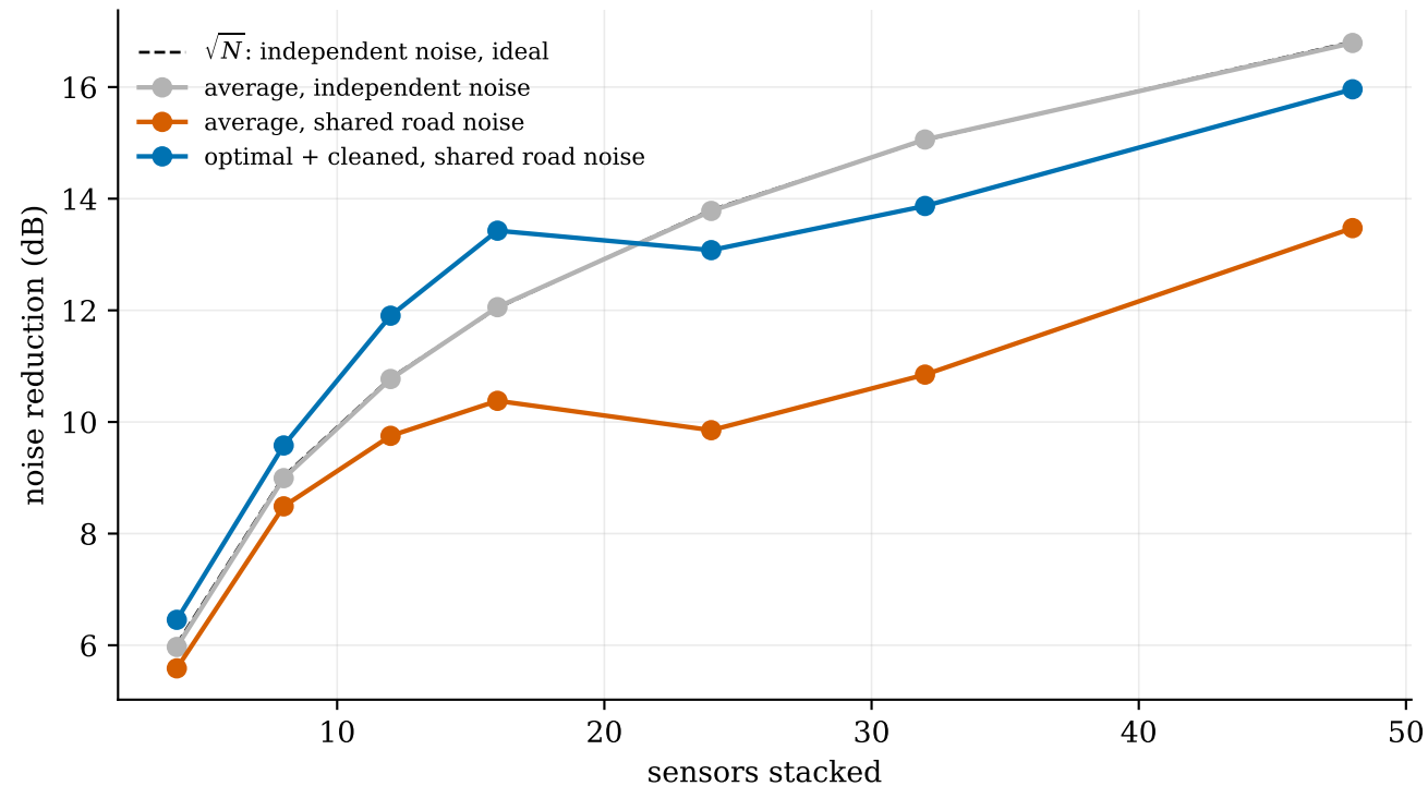
Shared noise defeats averaging; the covariance beats it
