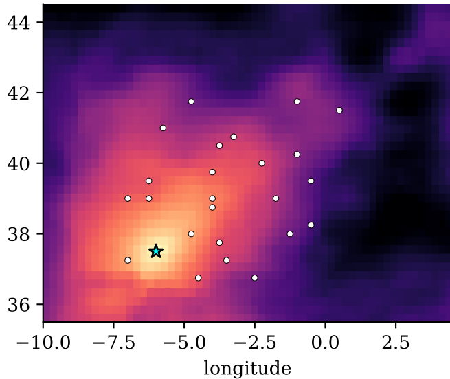
summer (JJA): correlation with Seville
