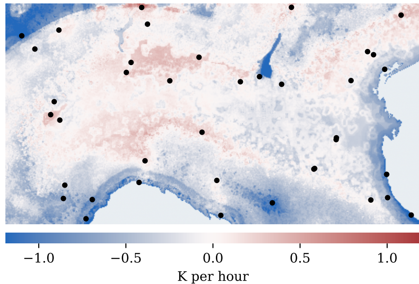
Mean missing heating q (dots are stations)
