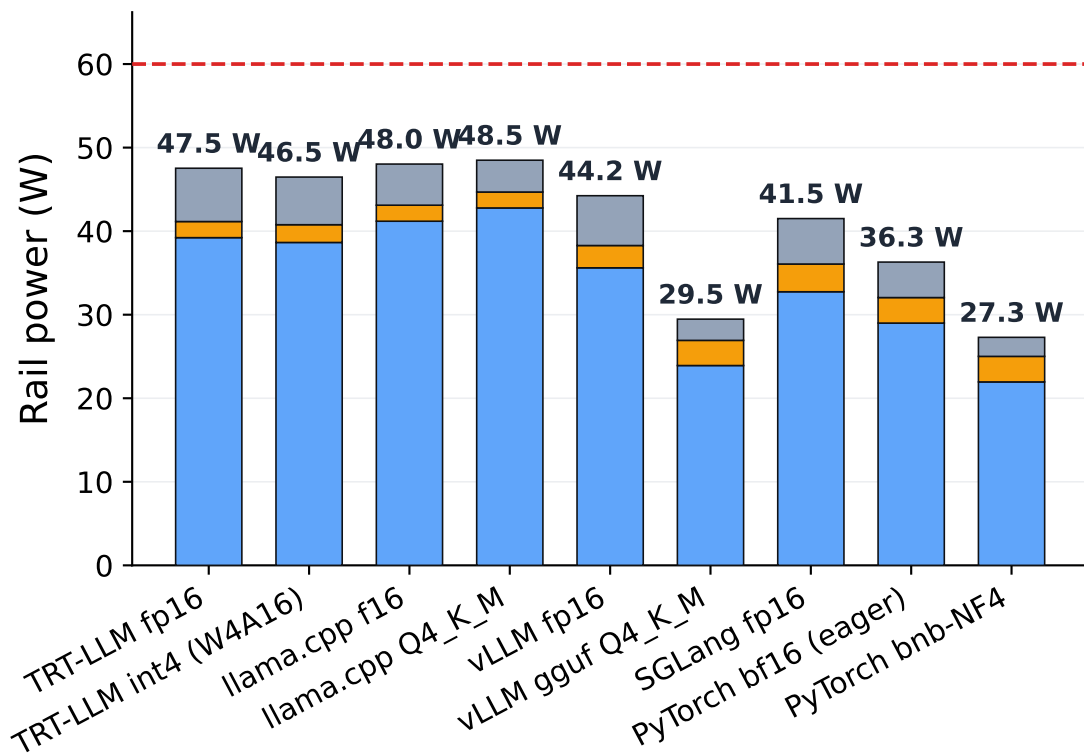
(c) Decode rail power
