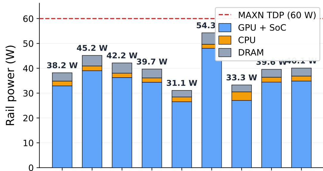
(a) Prefill rail power
