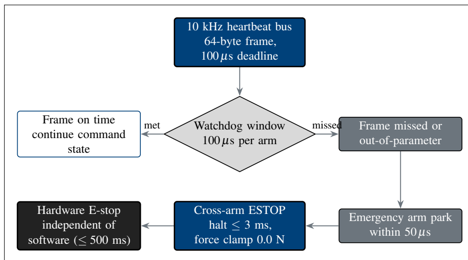
Figure 14. Heartbeat, watchdog, and E-stop architecture. A 10 kHz heartbeat bus with a 100 μs per-arm watchdog continues the command state on an on-time frame; a missed frame parks the arm within 50 μs and escalates to a cross-arm E-stop that halts the platform in \leq 3 ms at a 0.0 N force clamp, backed by a software-independent hardware E-stop meeting the §312.404 \leq 500 ms requirement.
