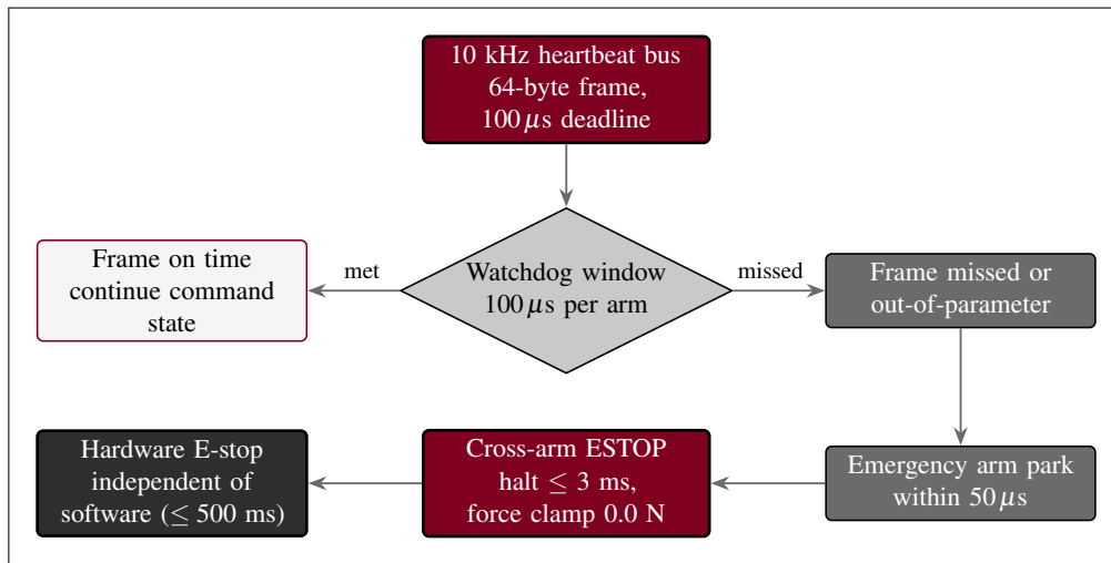
Figure 16. Heartbeat, watchdog, and E-stop architecture for Arm A. A 10 kHz heartbeat bus with a 100\mu\text{s} per arm watchdog continues the command state on an on-time frame; a missed frame parks the arm within 50\mu\text{s} and escalates to a cross-arm E-stop that halts the platform in \leq 3 ms at a 0.0 N force clamp, backed by a software-independent hardware E-stop meeting the \leq 500 ms requirement.
