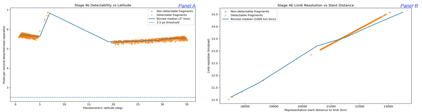
Figure 4b. Detectability diagnostics. Panel A shows fragment-level pixels per nominal detached-haze separation (76 km) as a function of planetocentric latitude for the processed .cub, with fragments classified as detectability-valid or geometry-limited relative to the adopted 2.5-pixel interpretability threshold. Panel B shows limb resolution (km per pixel) as a function of representative slant distance to the limb. These diagnostics separate geometry-limited fragments from geometry-valid non-detections prior to detached-haze occurrence aggregation and establish the retained interpretability structure inherited by downstream stages.
