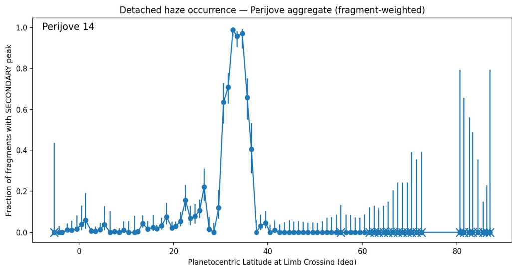
Figure 8.1 - Fragment-weighted detached haze occurrence vs. planetocentric latitude for Perijove 14, computed from the detectability-screened Stage 7 fragment population.
