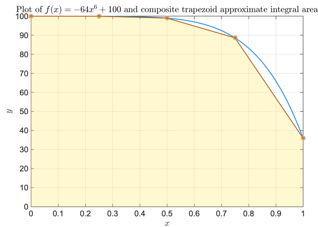
Figure 1: An example of numerical integration.
