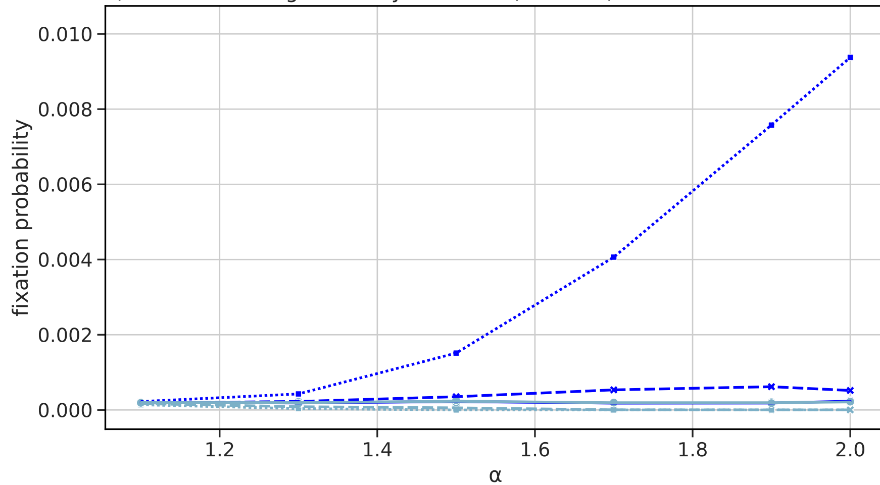
c) slow fluctuating fecundity selection (N=5000)
