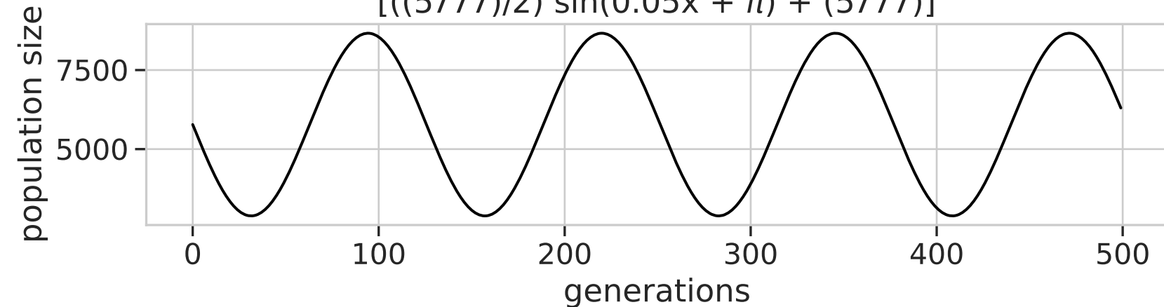
Fluctuating population size [ ((5777)/2) \sin(0.05x + \pi) + (5777) ]
