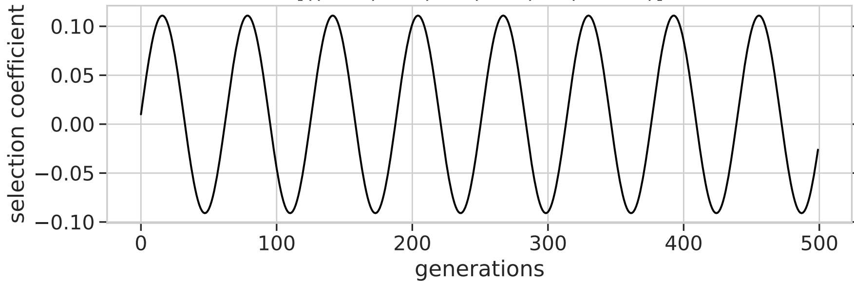
Fluctuating selection coefficient [ ((1.01)*0.1) \sin(0.1x) + (1.01-1) ]
