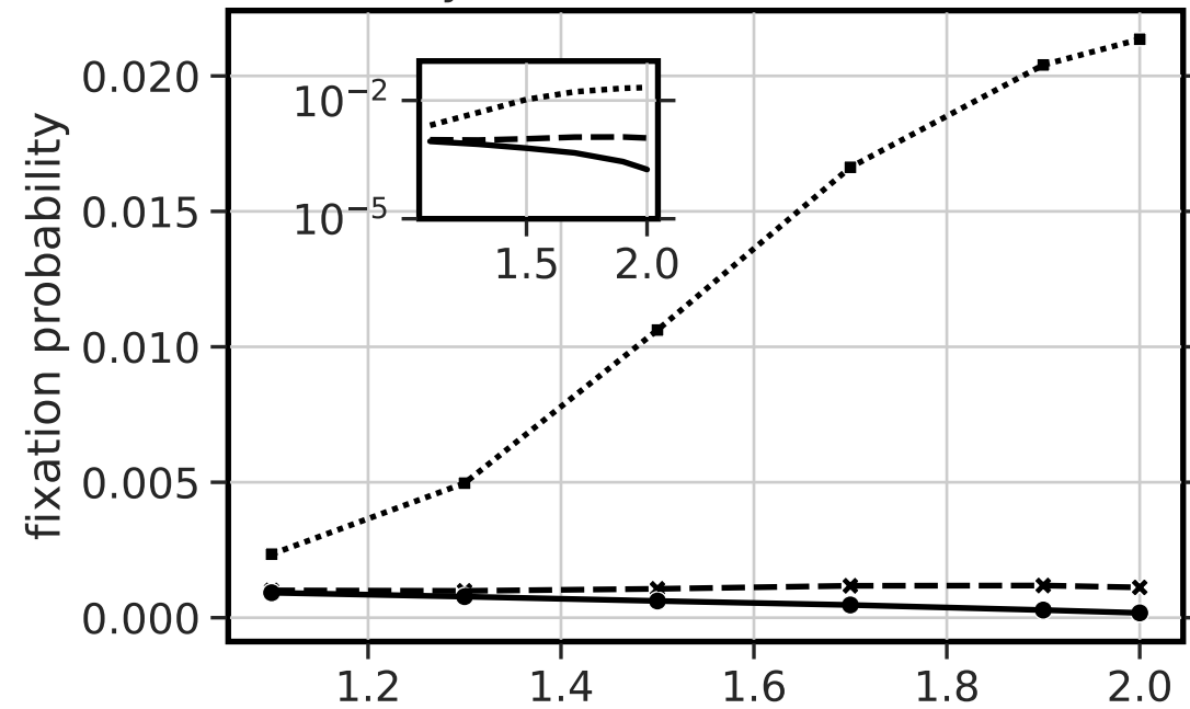
a) viability selection (N=1000)
