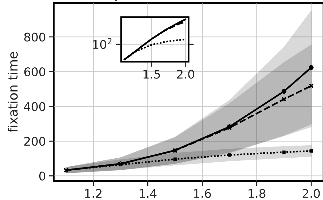
b) viability selection (N=1000)
