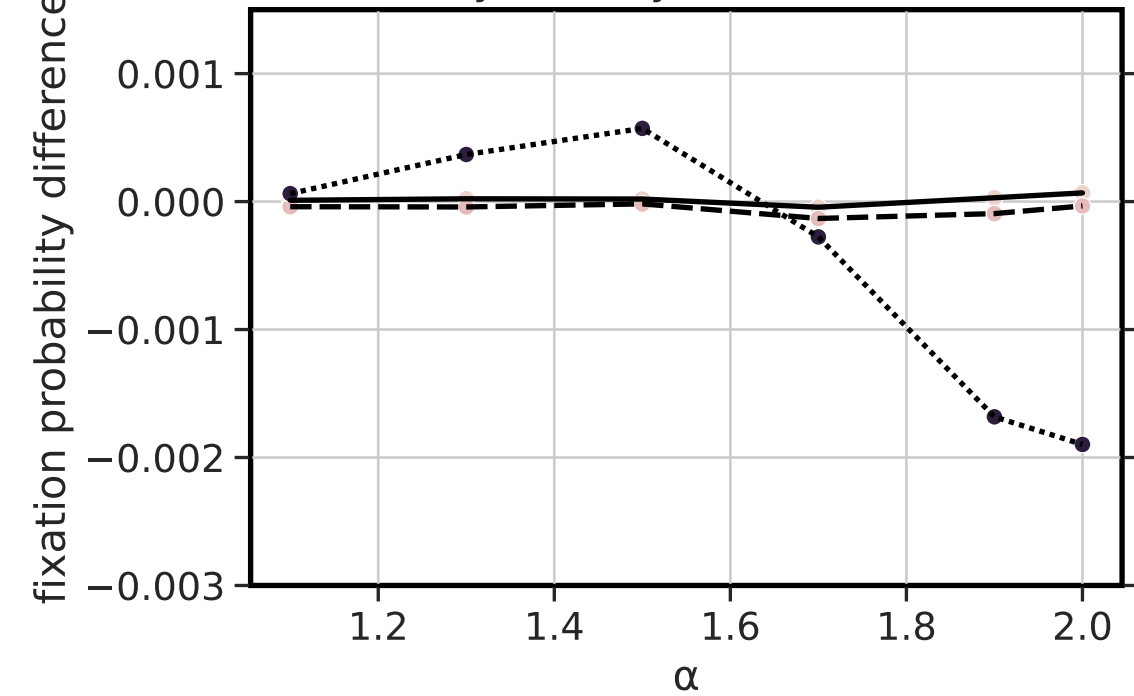
c) fecundity-viability selection (N=1000)
