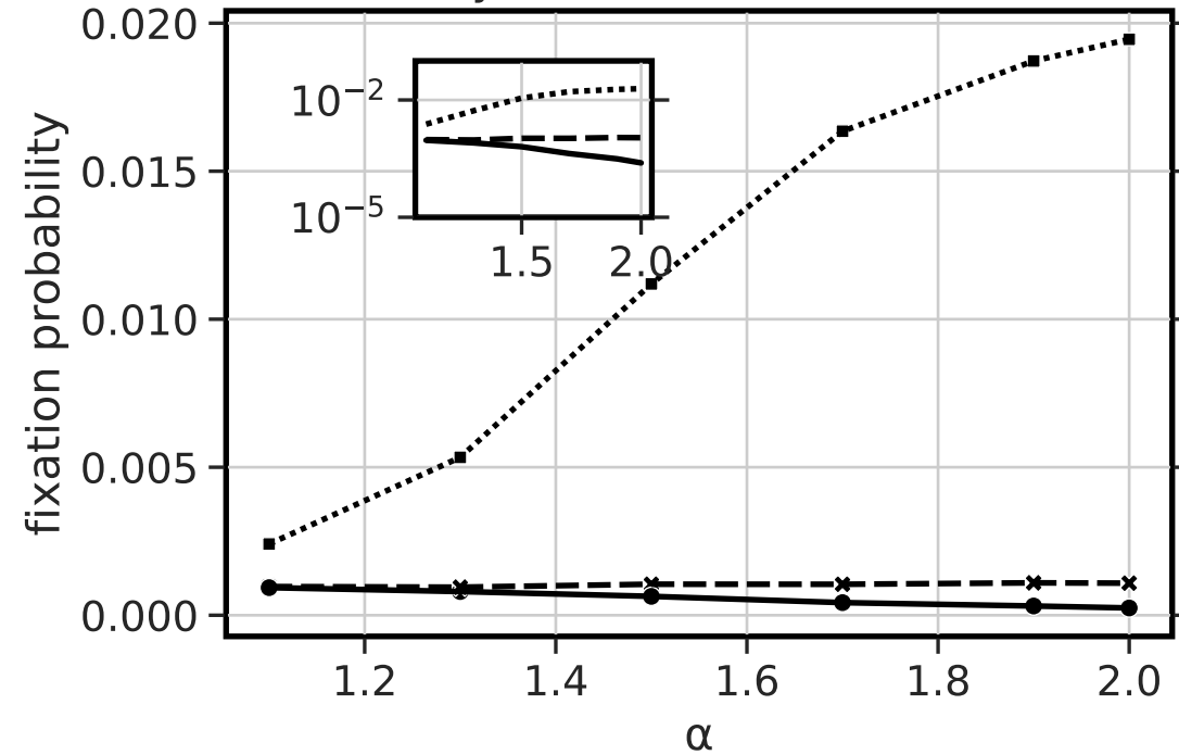
d) fecundity selection (N=1000)
