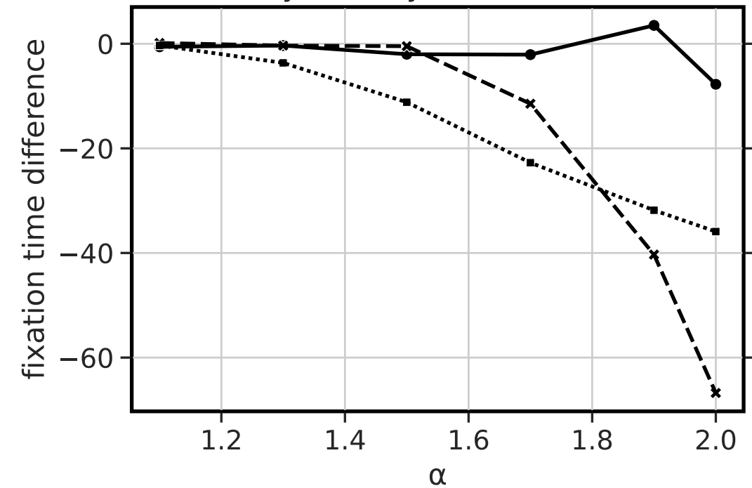
f) fecundity-viability selection (N=1000)
