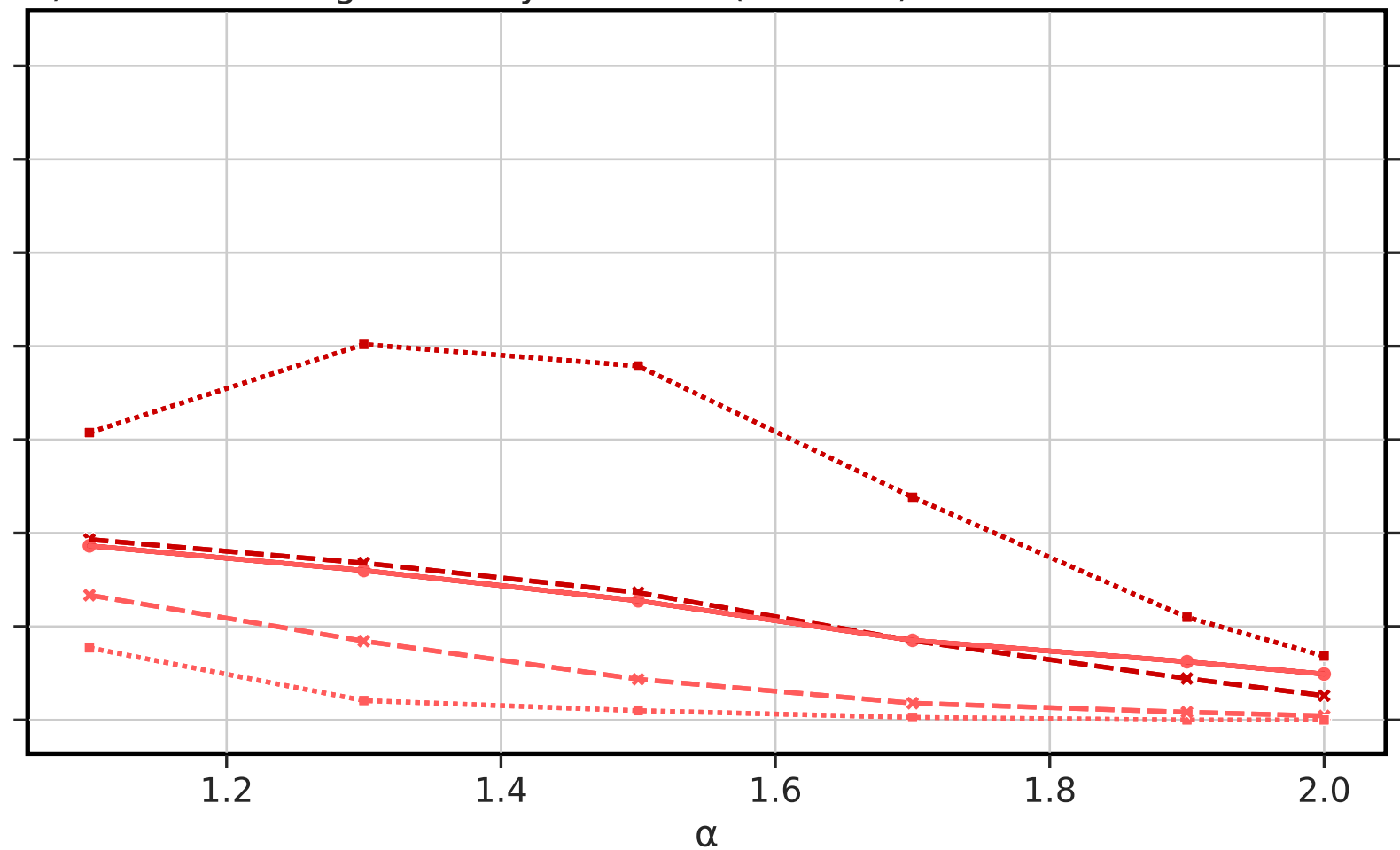
d) fast fluctuating fecundity selection (N=1000)
