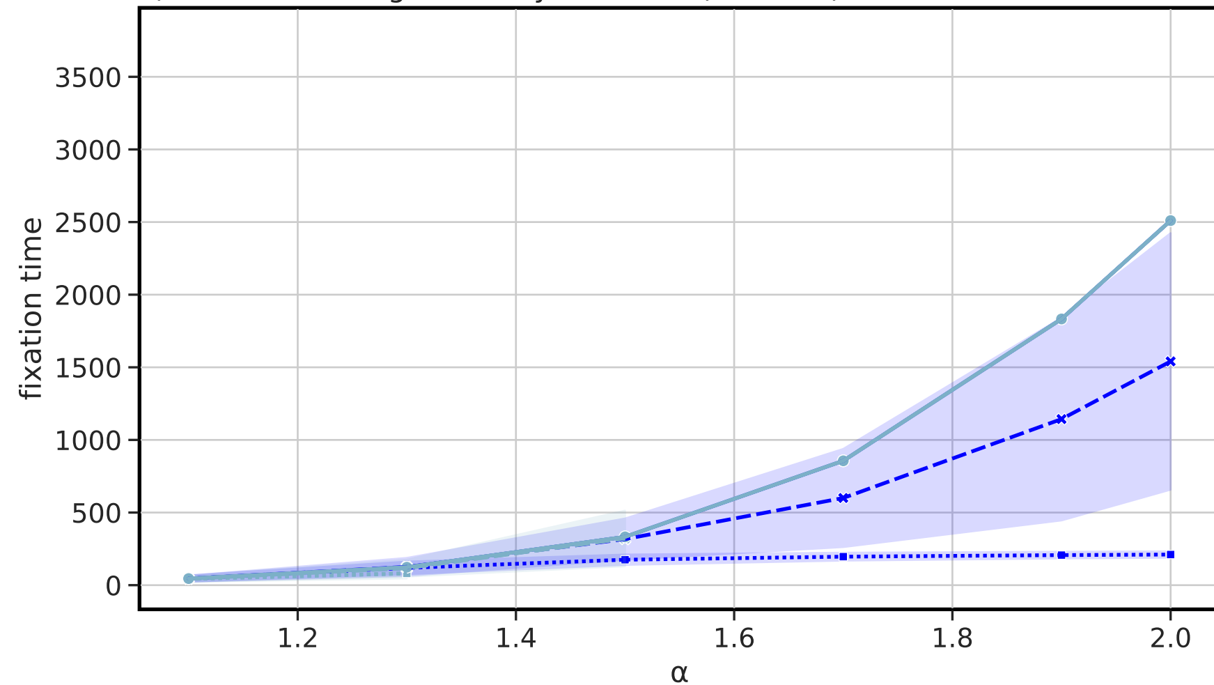
c) slow fluctuating fecundity selection (N=5000)
