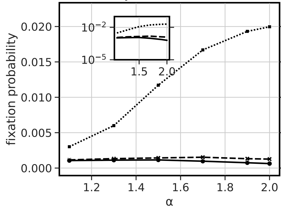
d) fecundity selection (N=578)
