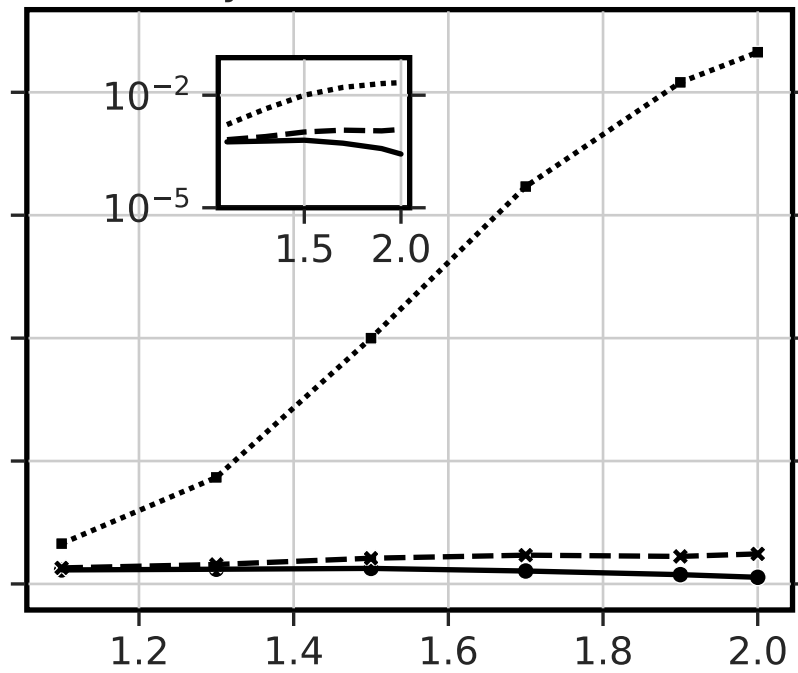
b) viability selection (N=1156)
