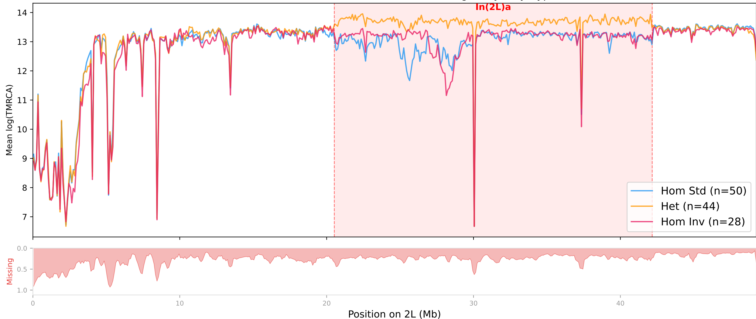
Guinea — Intra-individual coalescence along 2L by karyotype
