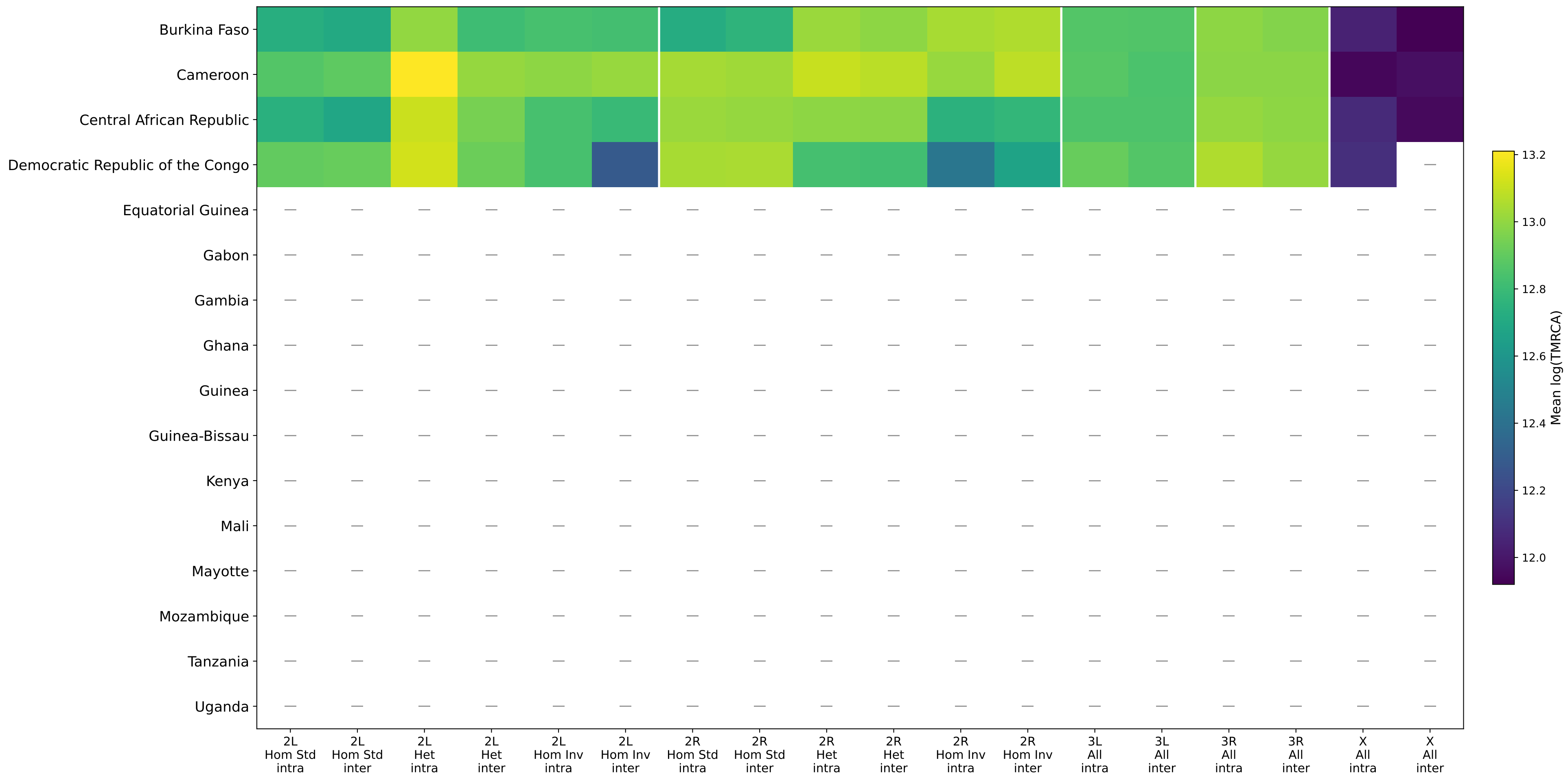
Mean coalescence time — all populations × karyotype groups × pair types
