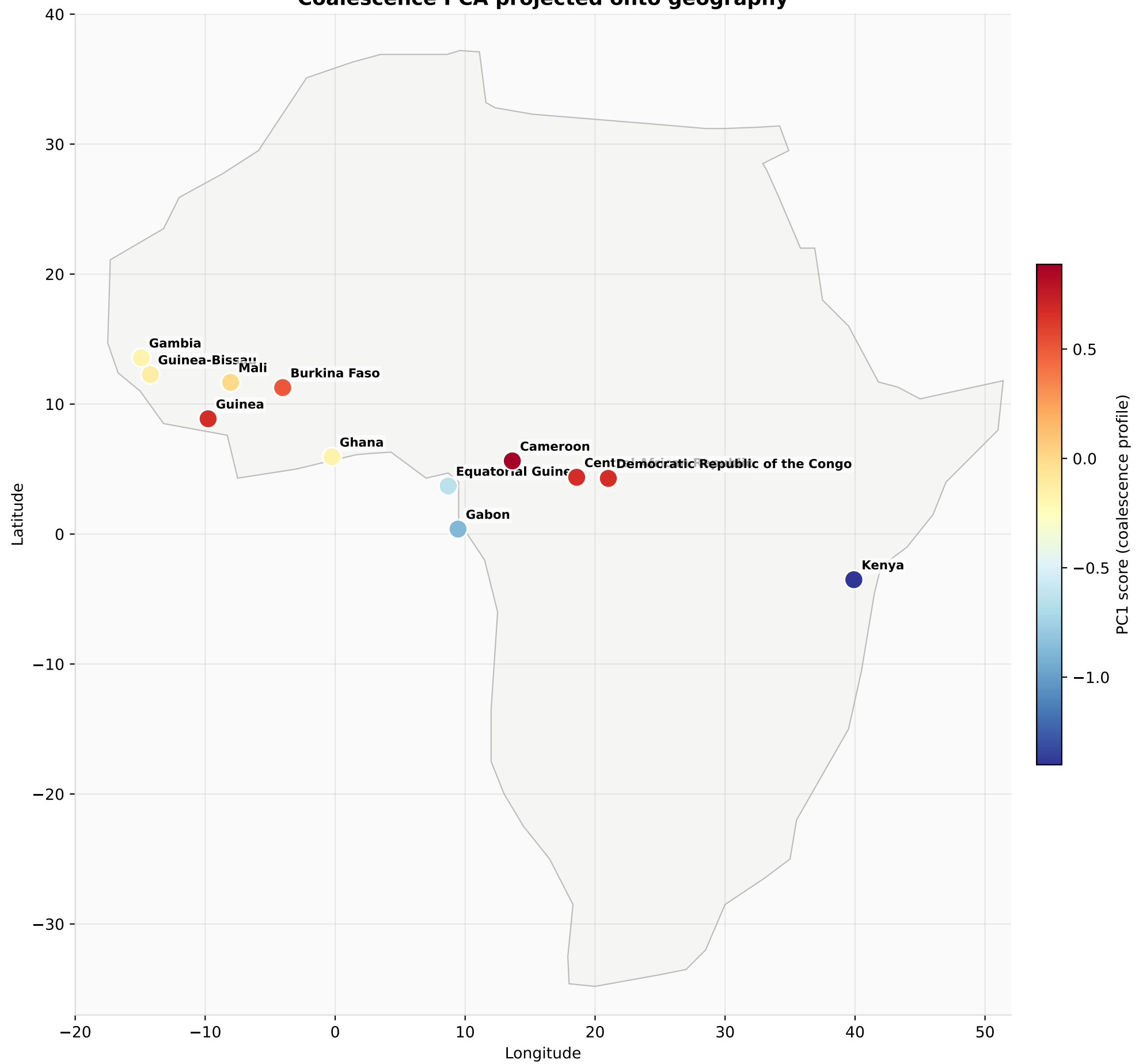
Coalescence PCA projected onto geography
