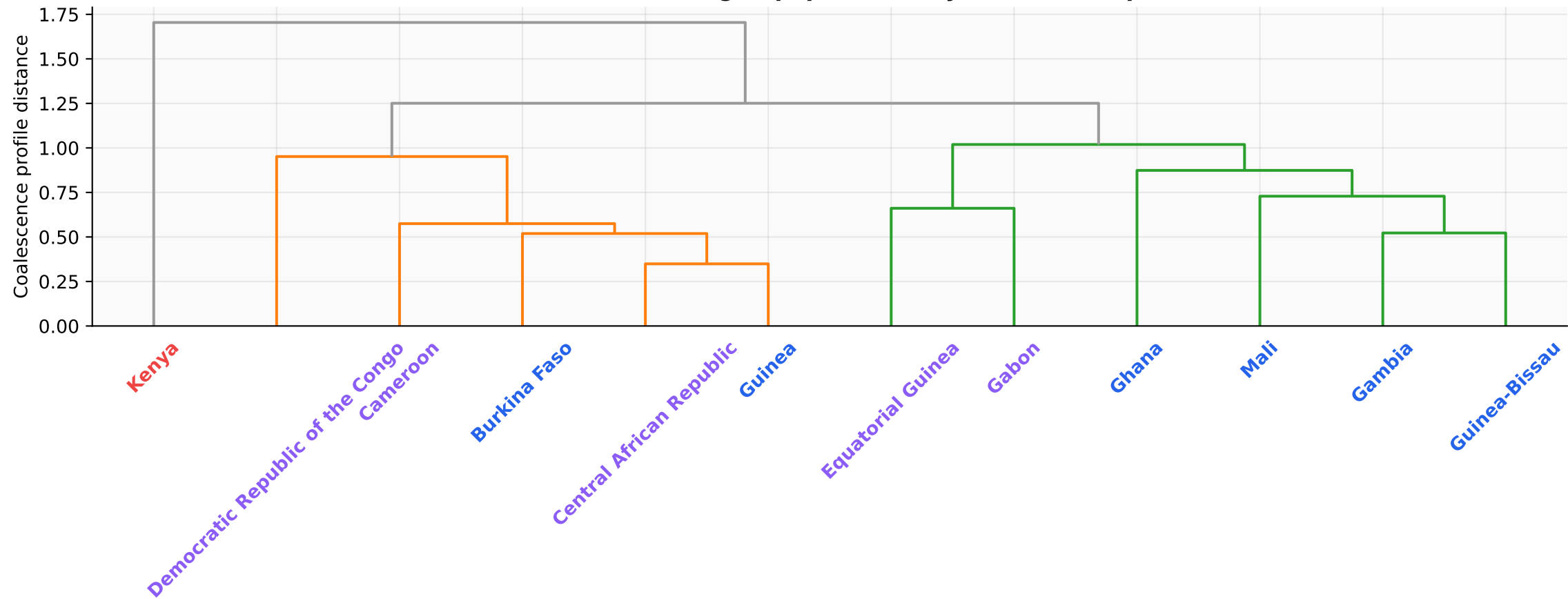
Hierarchical clustering of populations by coalescence profile
