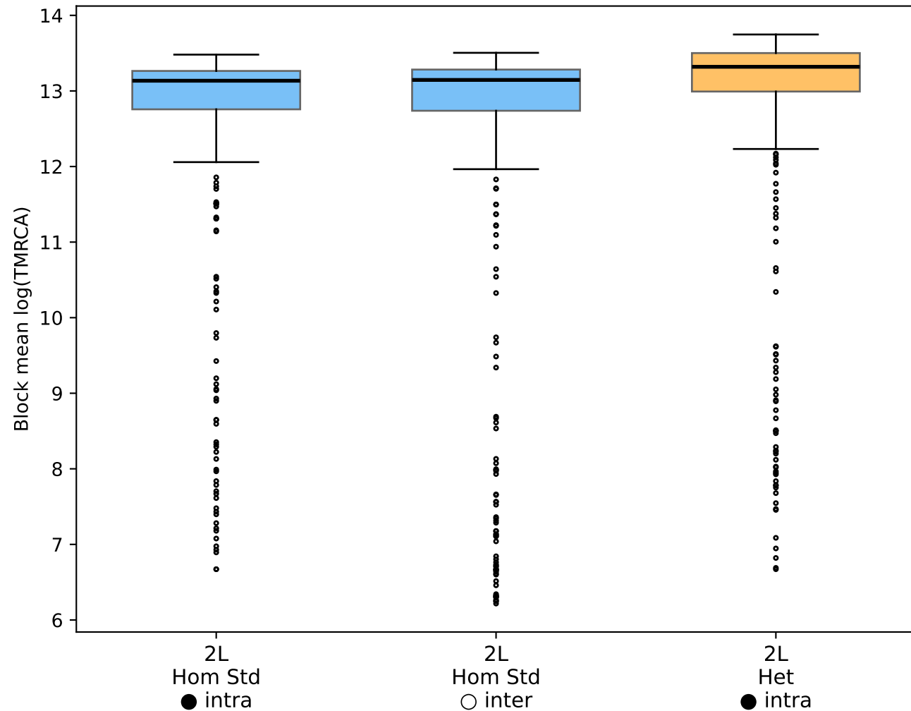
Guinea-Bissau — Coalescence by karyotype group and pair type
