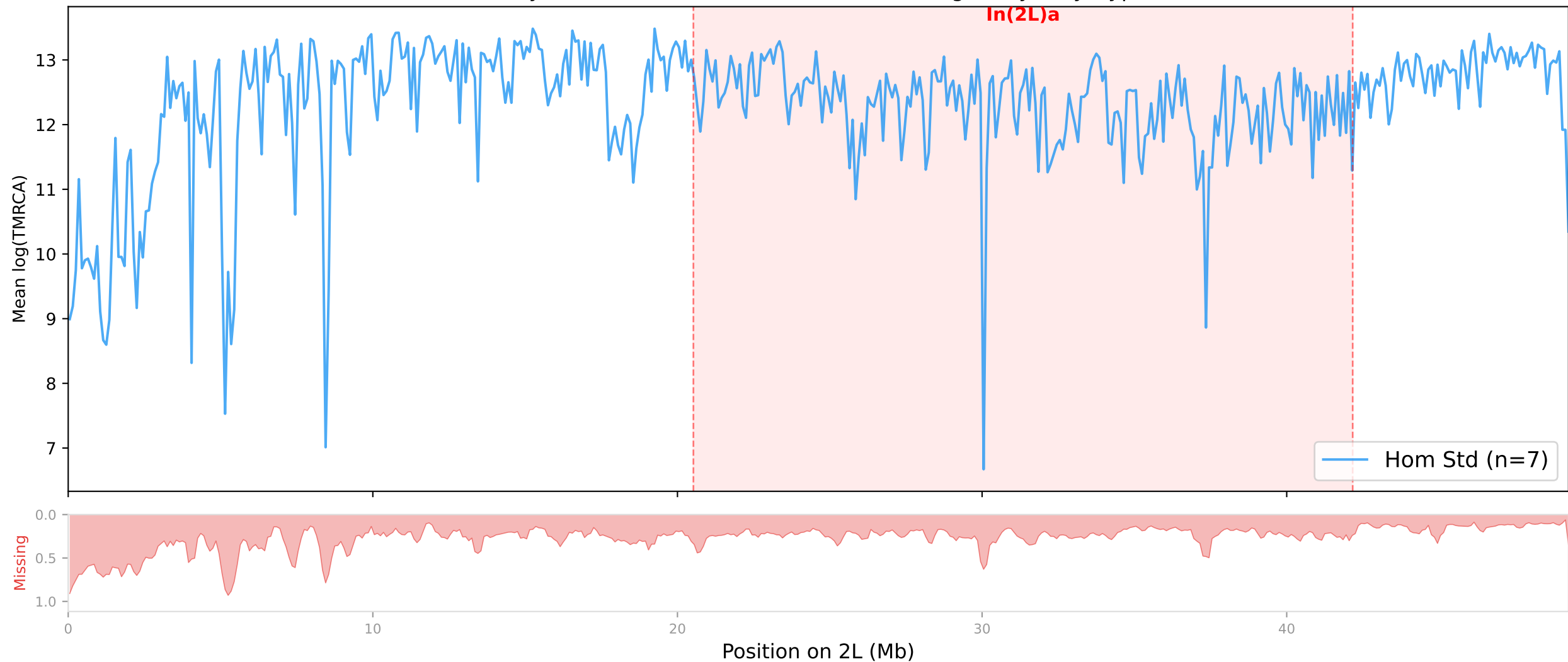
Kenya — Intra-individual coalescence along 2L by karyotype
