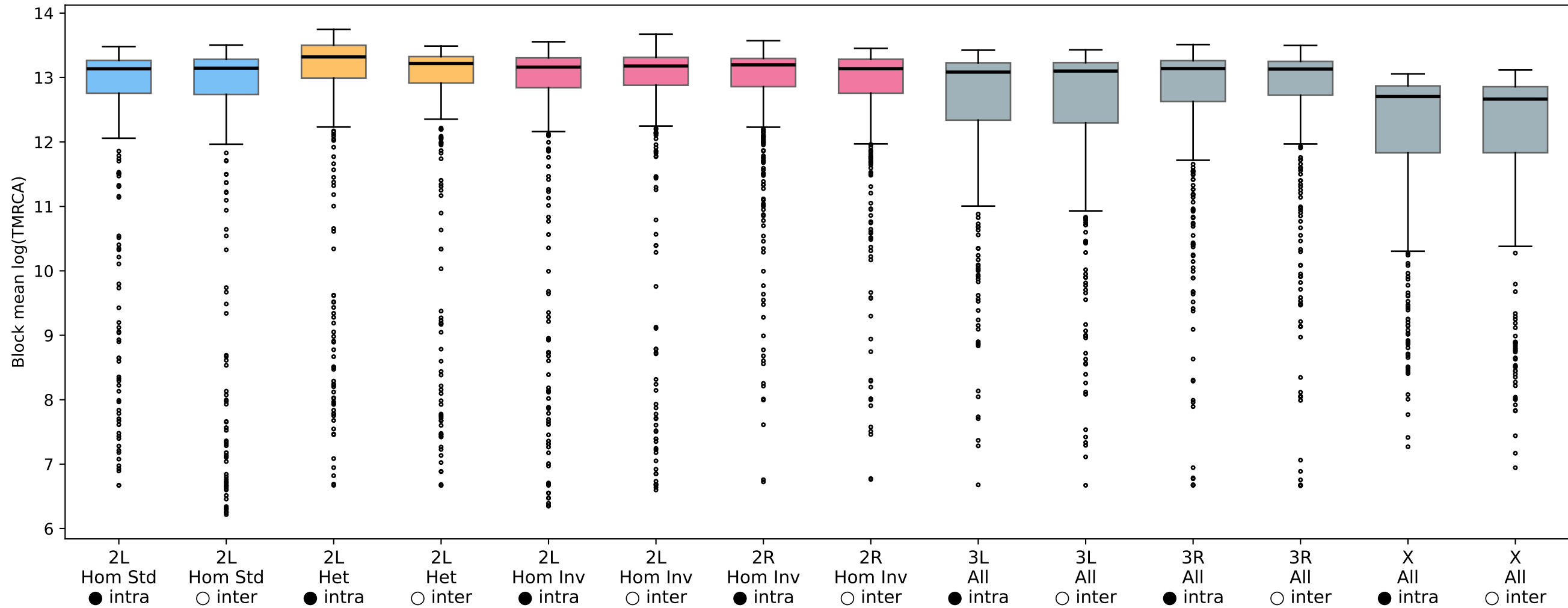
Guinea-Bissau — Coalescence by karyotype group and pair type
