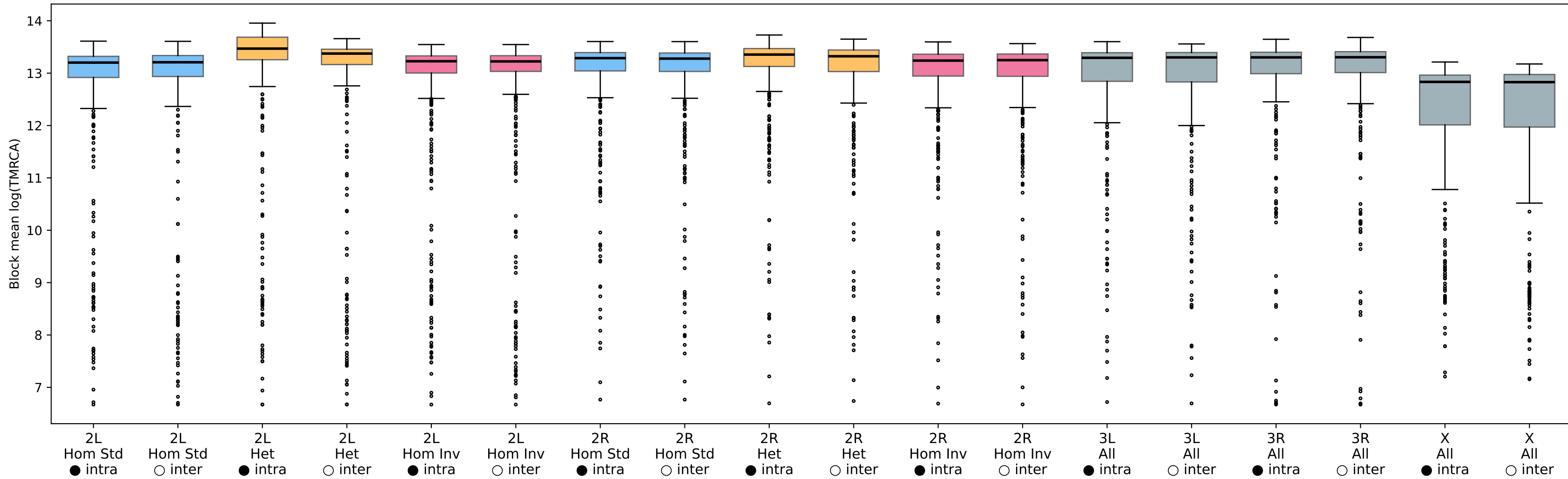
Guinea — Coalescence by karyotype group and pair type
