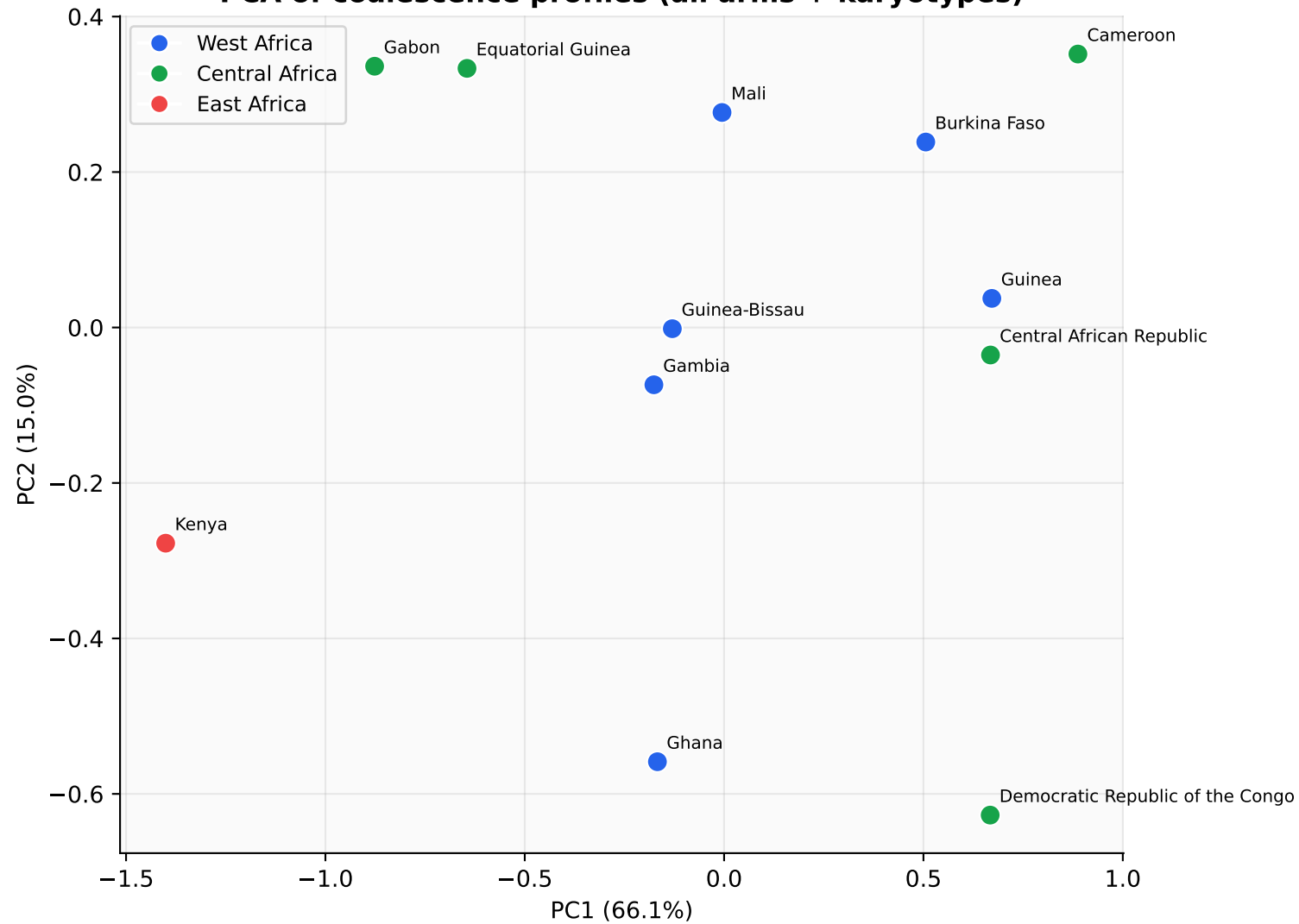
PCA of coalescence profiles (all arms + karyotypes)
