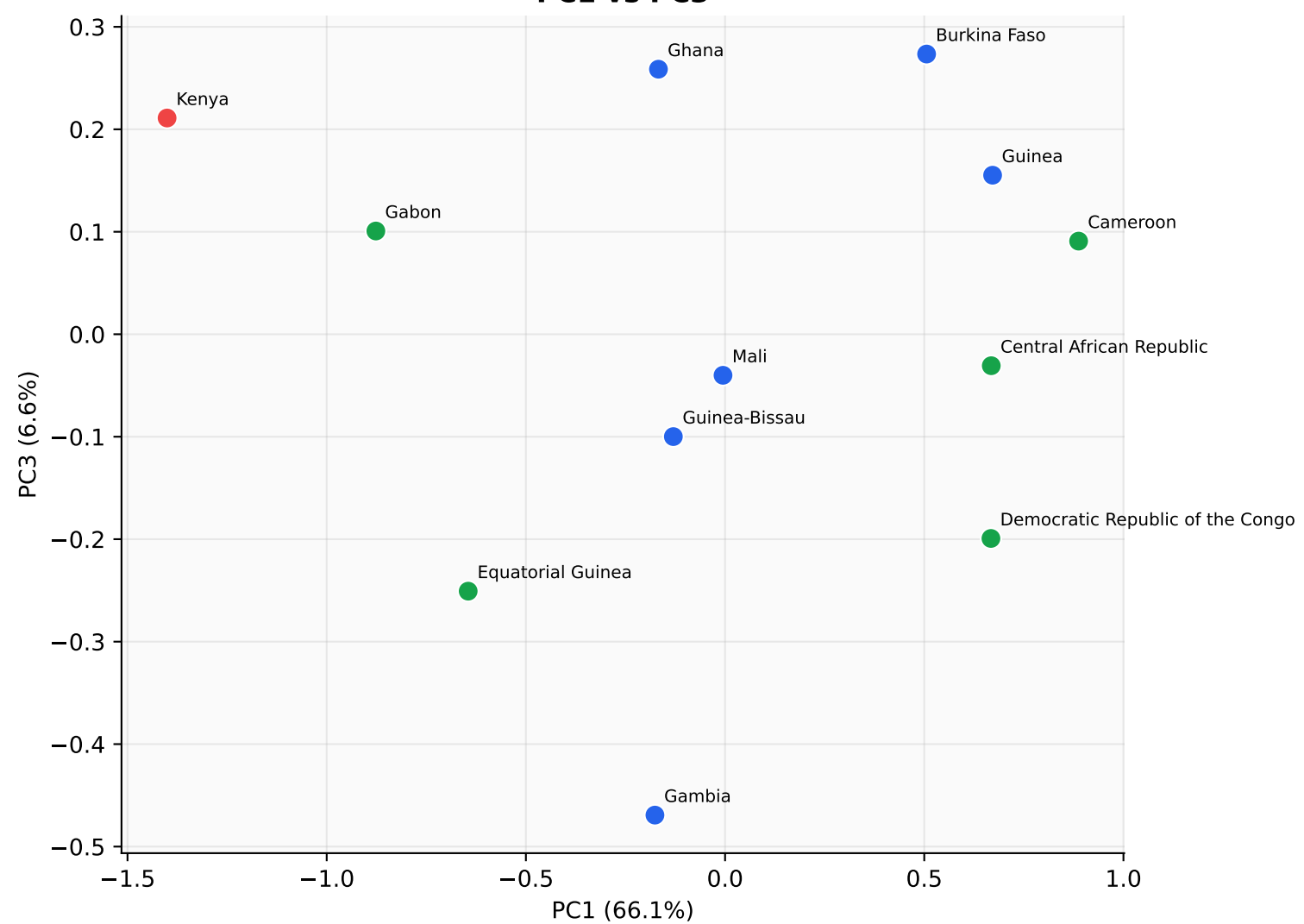
PC1 vs PC3
