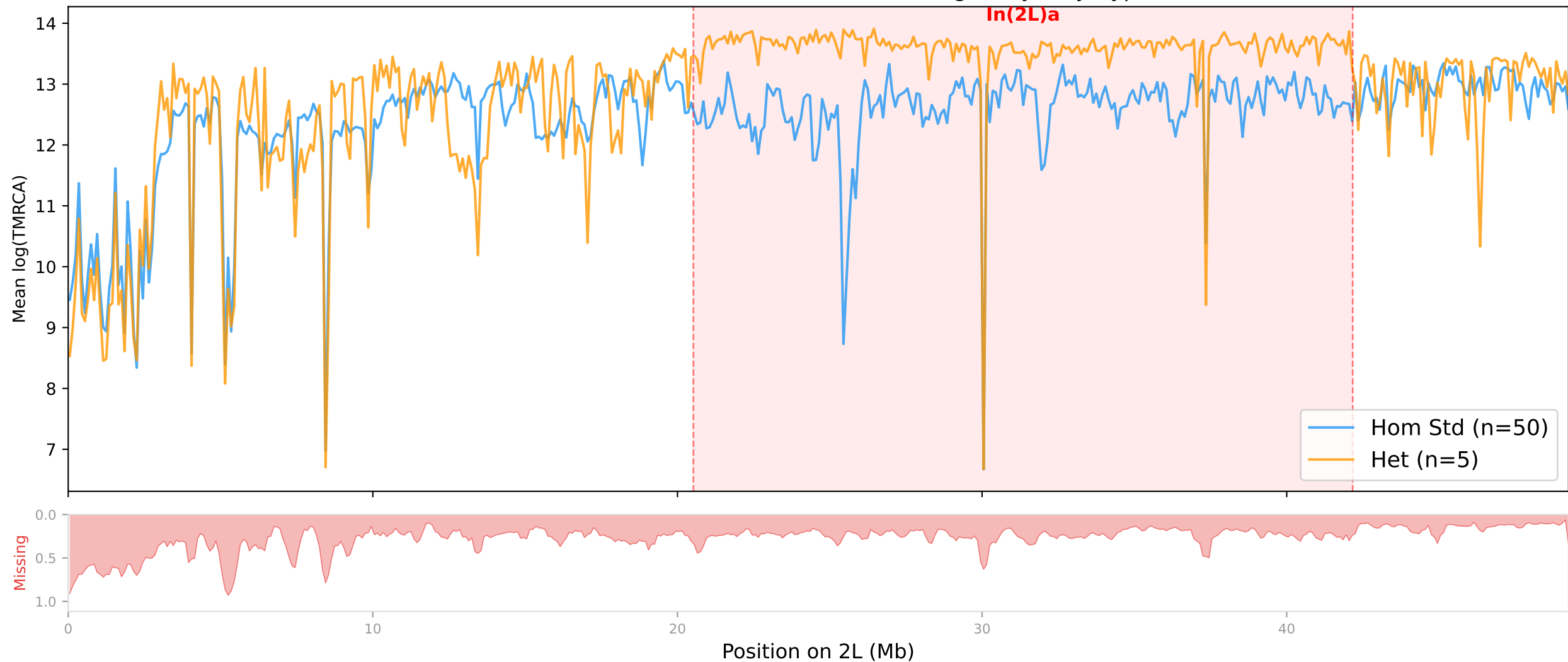
Gabon — Intra-individual coalescence along 2L by karyotype
