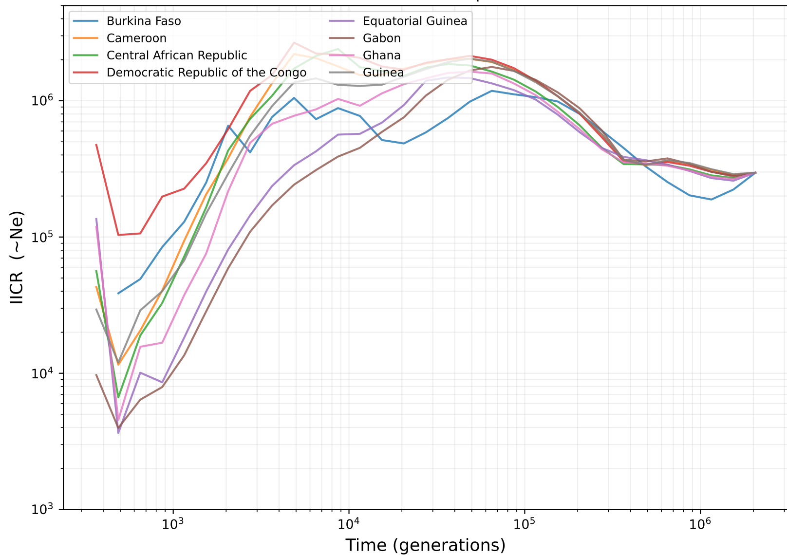
Demographic inference — 2L Hom Std intra
