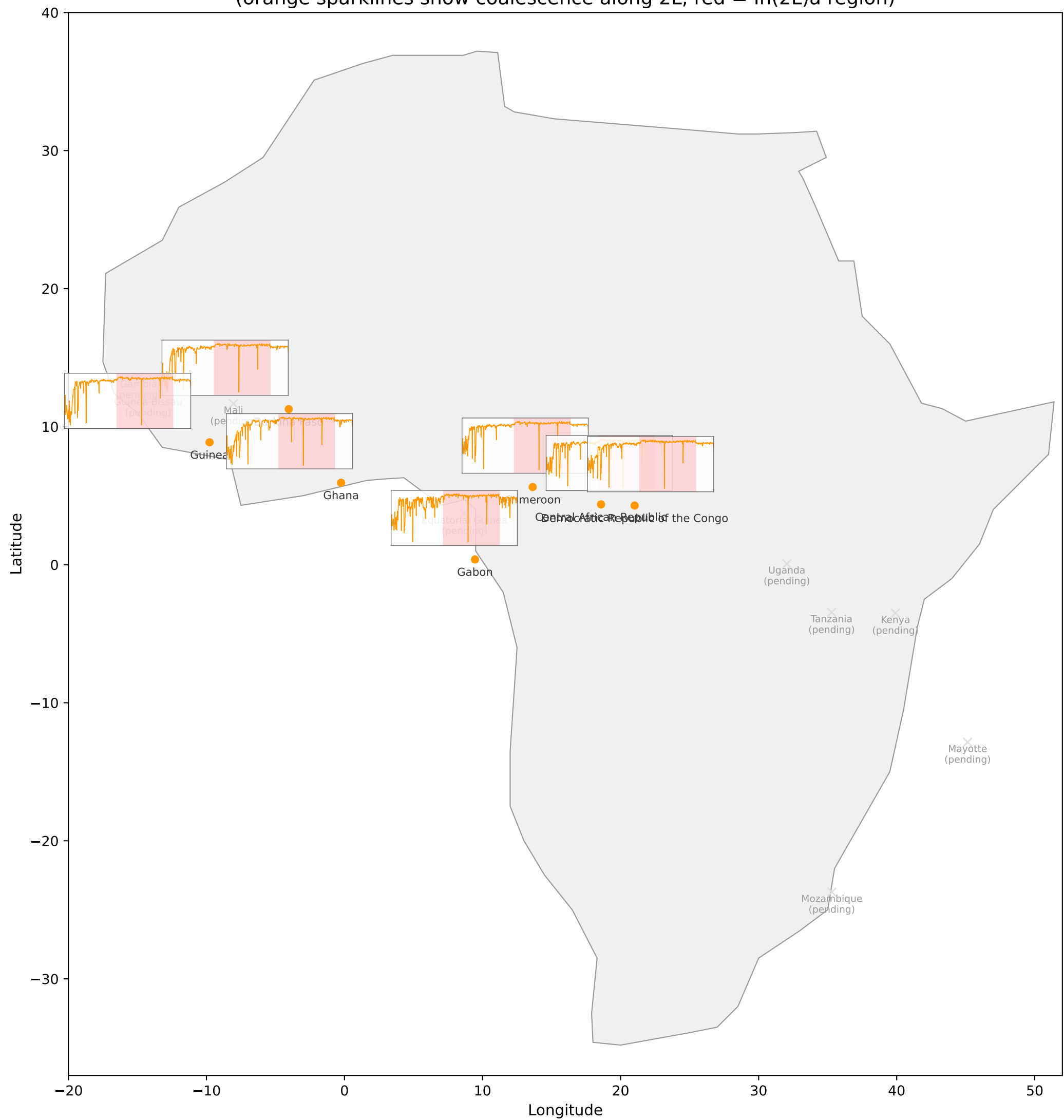
2L heterozygous — intra-individual TMRCA profiles across Africa (orange sparklines show coalescence along 2L, red = \ln(2L)_a region)
