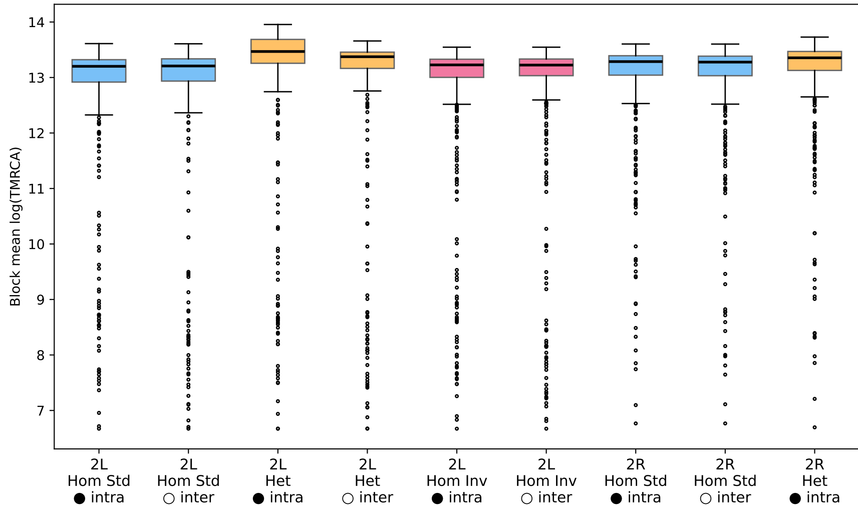
Guinea — Coalescence by karyotype group and pair type
