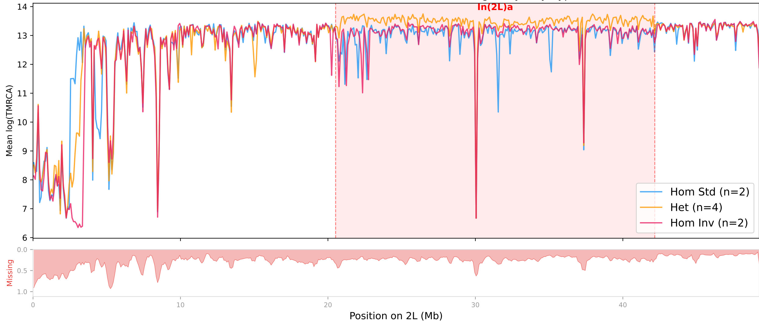
Guinea-Bissau — Intra-individual coalescence along 2L by karyotype
