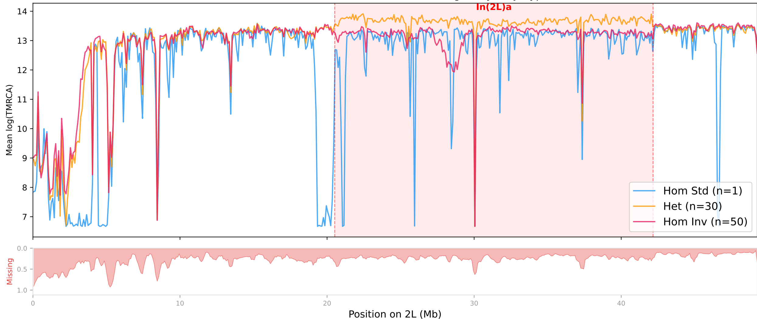
Mali — Intra-individual coalescence along 2L by karyotype
