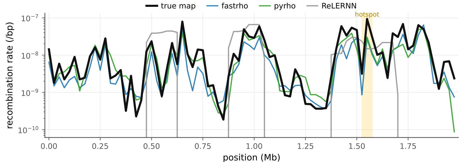
Example inferred map (real HapMap region): fastrho tracks the truth at fine scale
