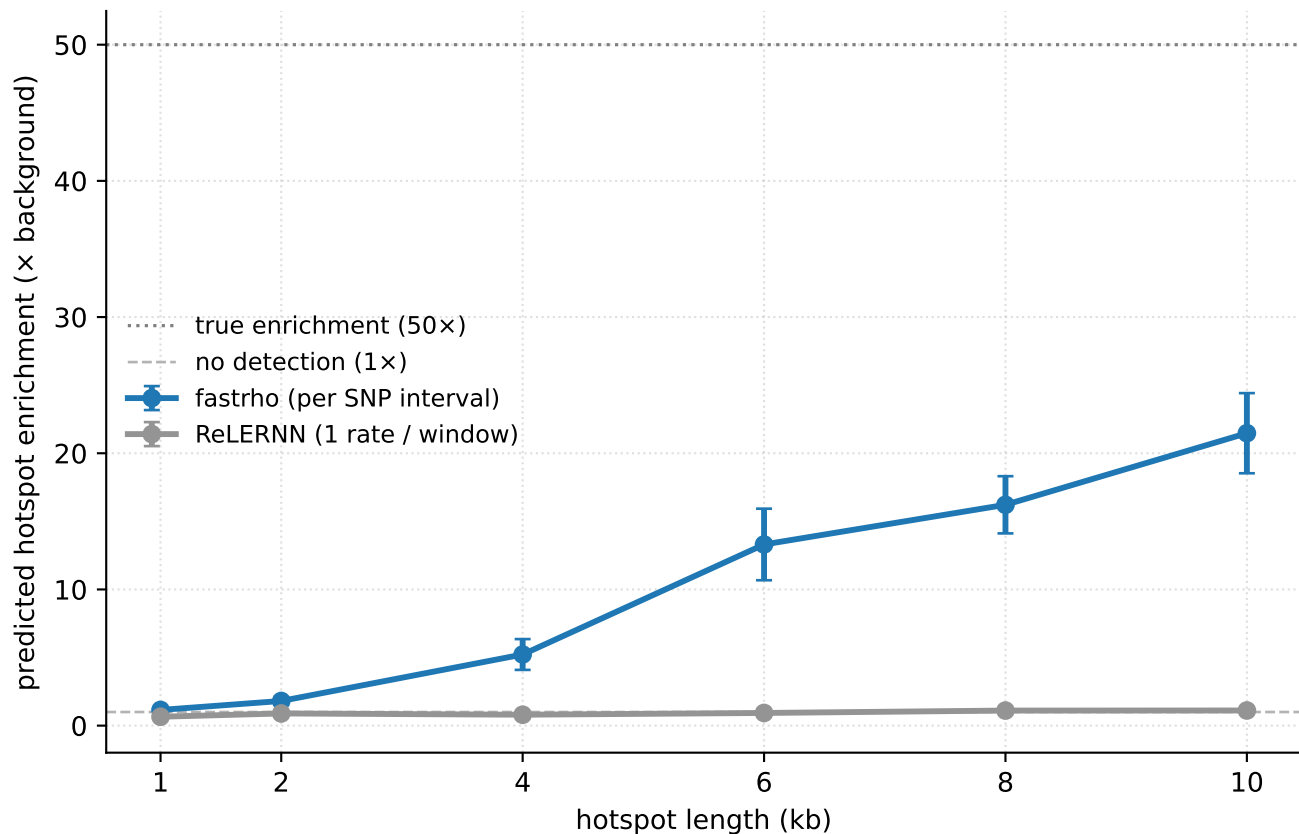
Detecting short hotspots: fastrho resolves what ReLERNN cannot (ReLERNN SI Fig. S13 setup: 250 kb region, 50 \times hotspot, n = 20 )
