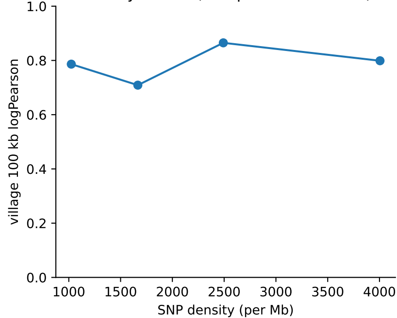
density-robust (real panel \sim 7800/\text{Mb} )
