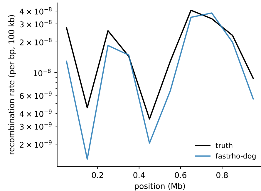
village region (logPearson=0.96)
