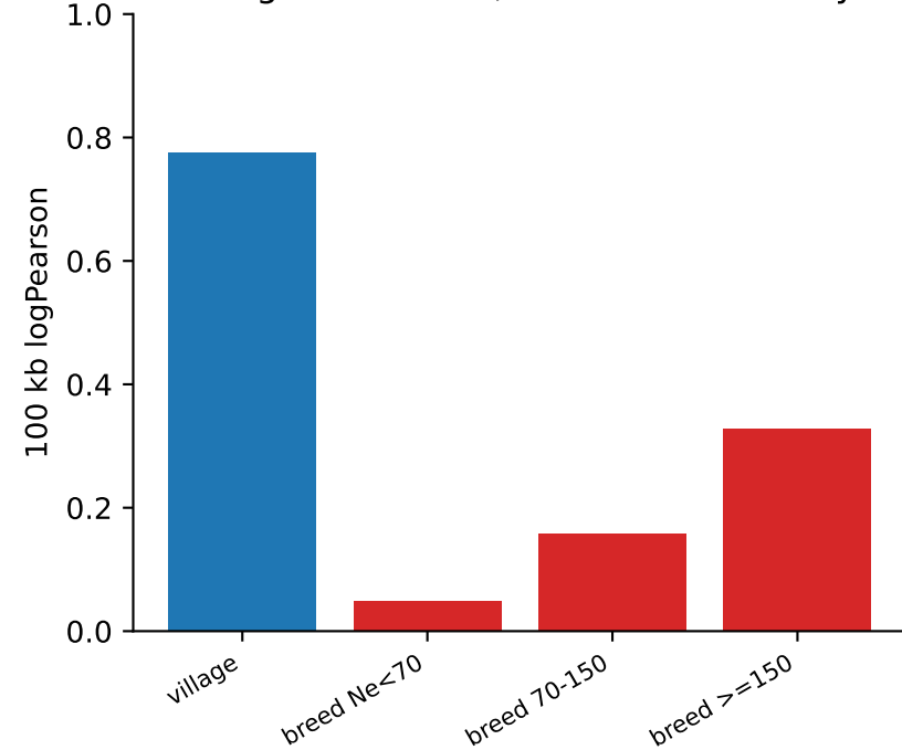
village resolvable; breed transfer-only
