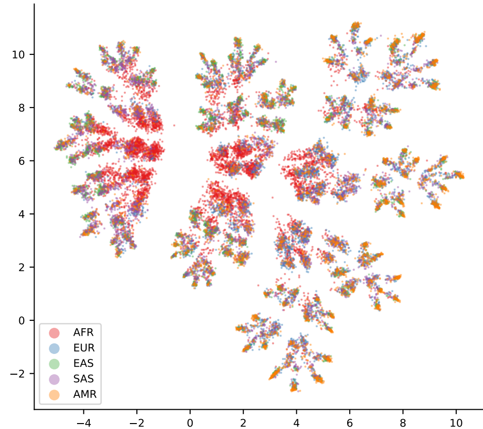
All genes, unsupervised
