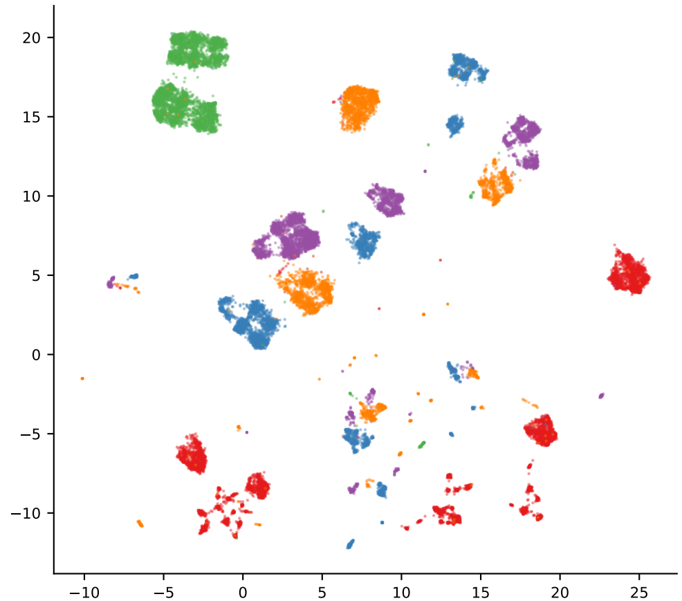
Outlier genes, supervised (5 superpopulations)
