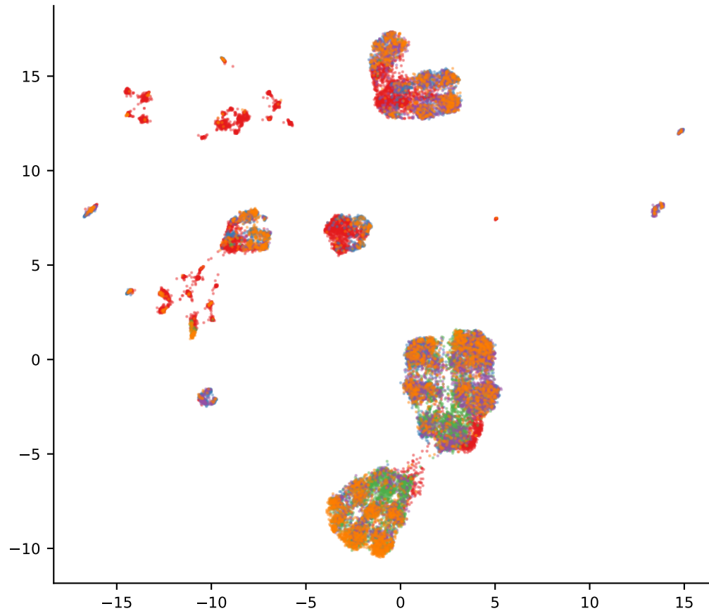
Outlier genes, unsupervised
