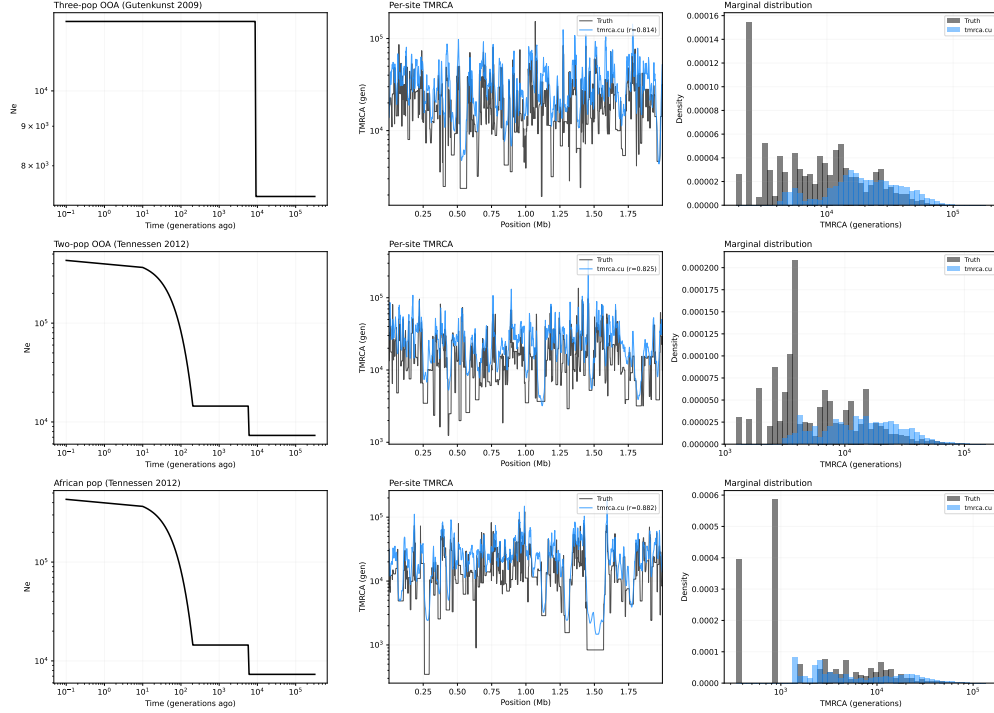
Figure 6: Demographic robustness. Three demographic models from stdpopsim : Gutenkunst et al. out-of-Africa (top), Tennessen et al. two-population (middle), and Tennessen et al. African population (bottom). Left: effective population size history. Centre: per-site TMRCA traces (black: truth; blue: tmrca.cu ). Right: marginal TMRCA distribution. The constant- N_e flow field was used in all cases; accuracy is maintained across diverse demographic histories ( r = 0.82 – 0.88 ).
