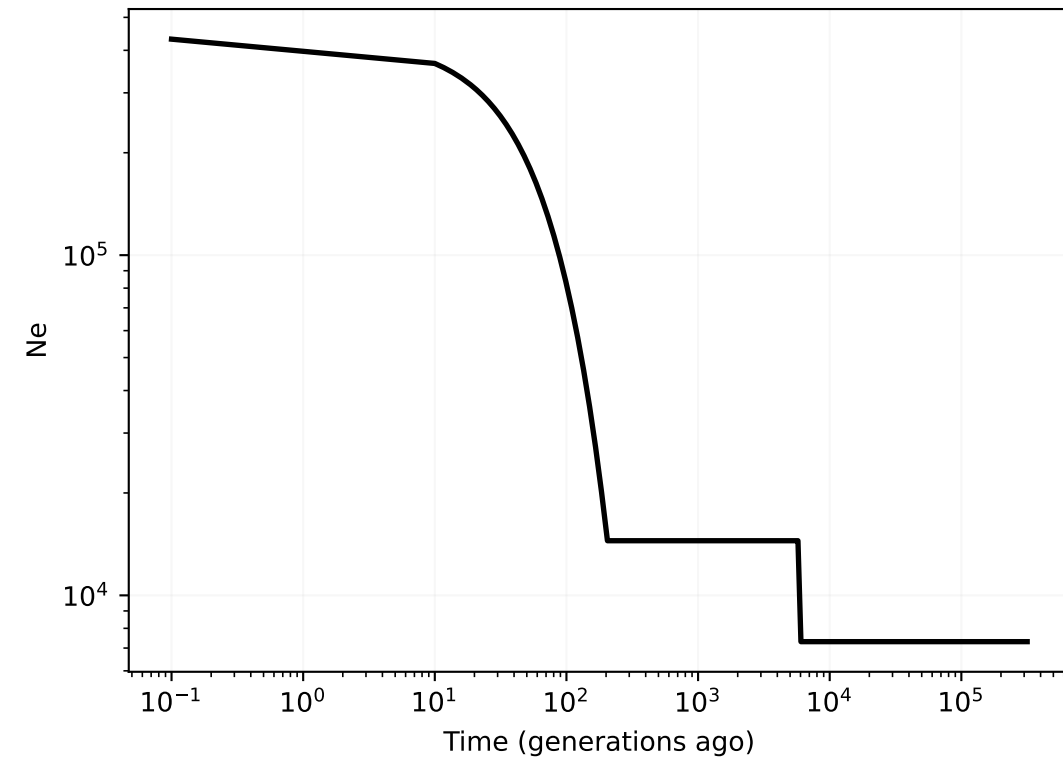
African pop (Tennessen 2012)
