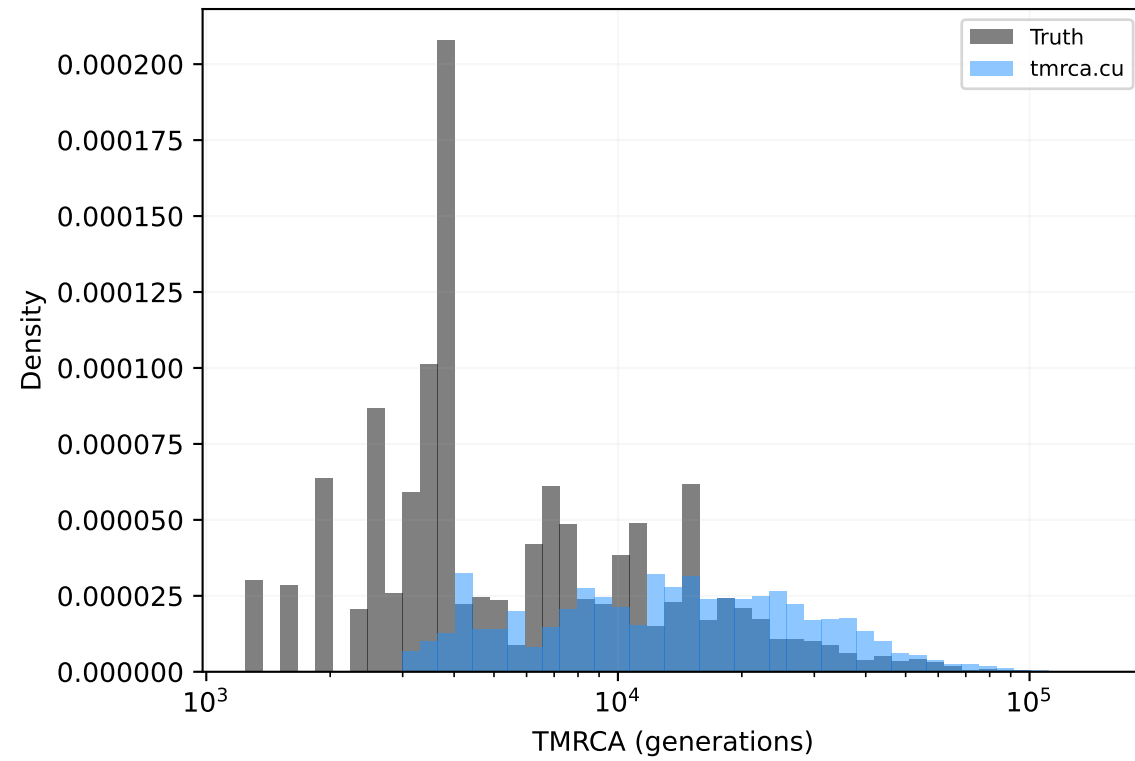
Marginal distribution
