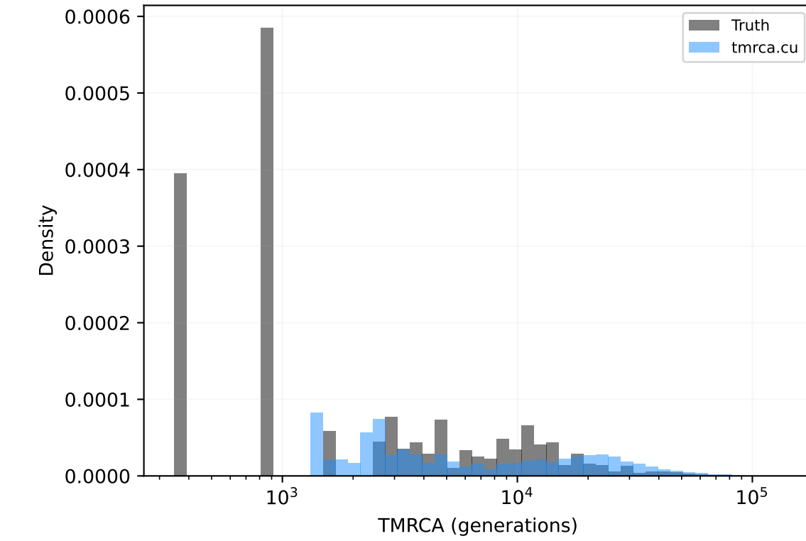
Marginal distribution
