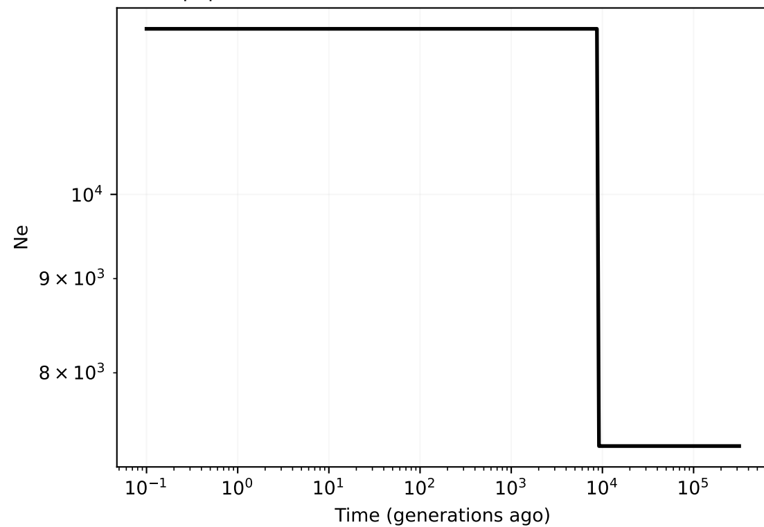
Two-pop OOA (Tennessen 2012)
