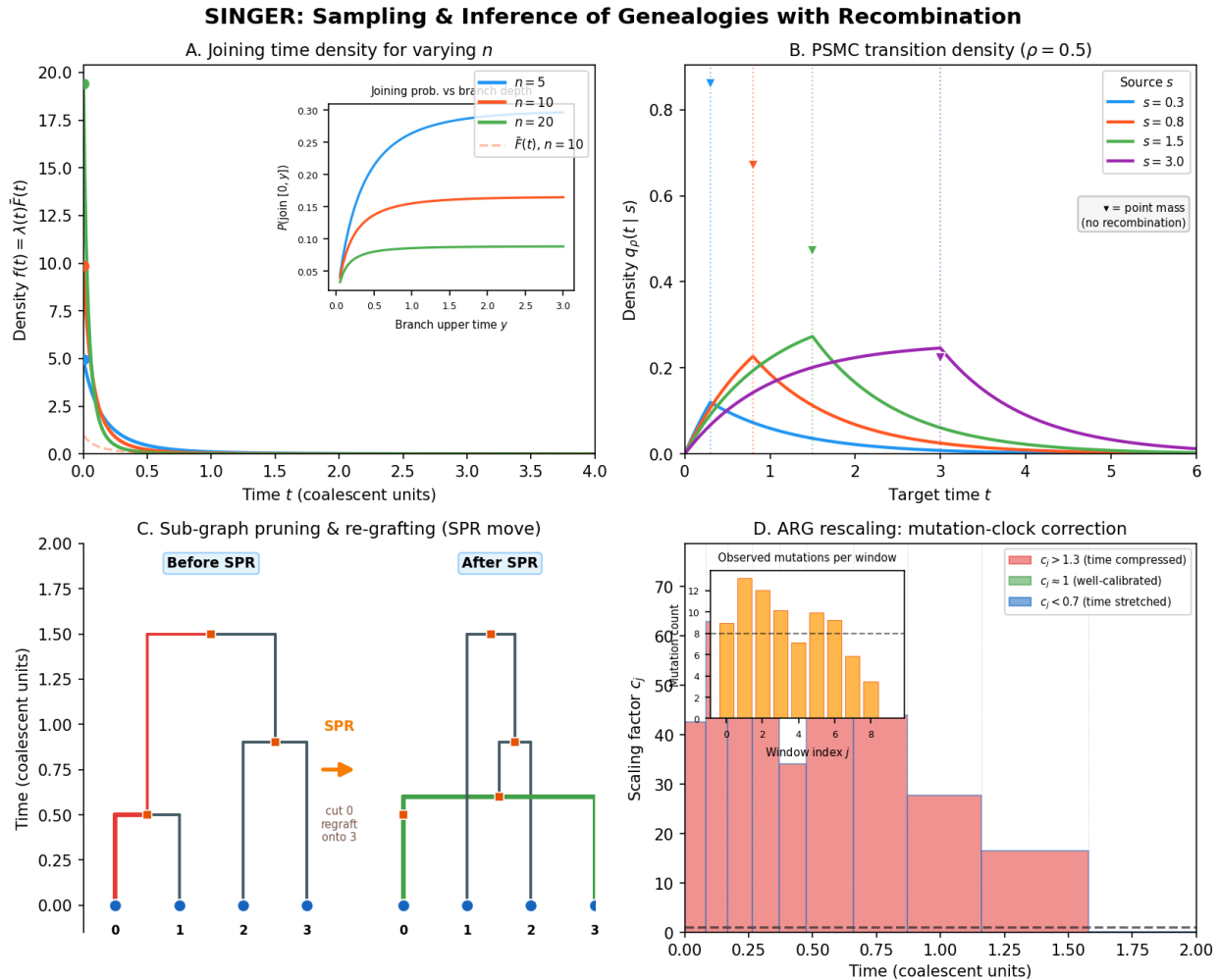
Fig. 13: SINGER at a glance. The four key gears of the SINGER algorithm: branch joining probabilities governing how lineages merge in the ARG, PSMC transition densities reused from Timepiece I for the pairwise coalescence kernel, SPR (subtree prune and regraft) tree rearrangement showing how MCMC proposals modify the genealogy, and ARG rescaling factors that adjust branch lengths to match the data.
