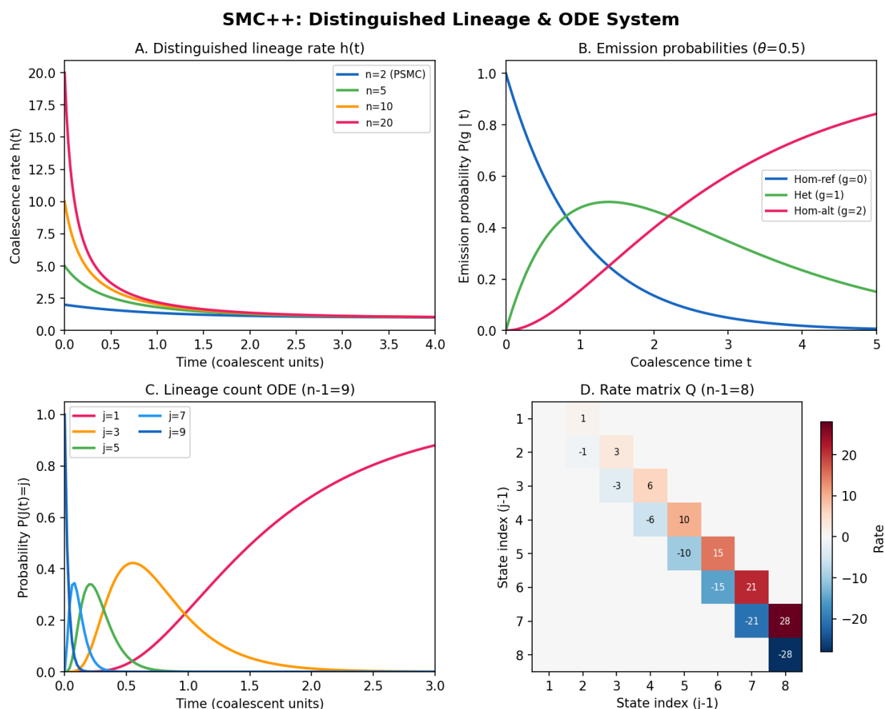
Fig. 3: SMC++ at a glance. The distinguished-lineage approach to multi-sample demographic inference: coalescence rate h(t) for varying sample sizes, emission probabilities linking hidden states to observations, ODE lineage-count evolution tracking how many lineages remain at each time, and the rate matrix structure that drives the HMM.
