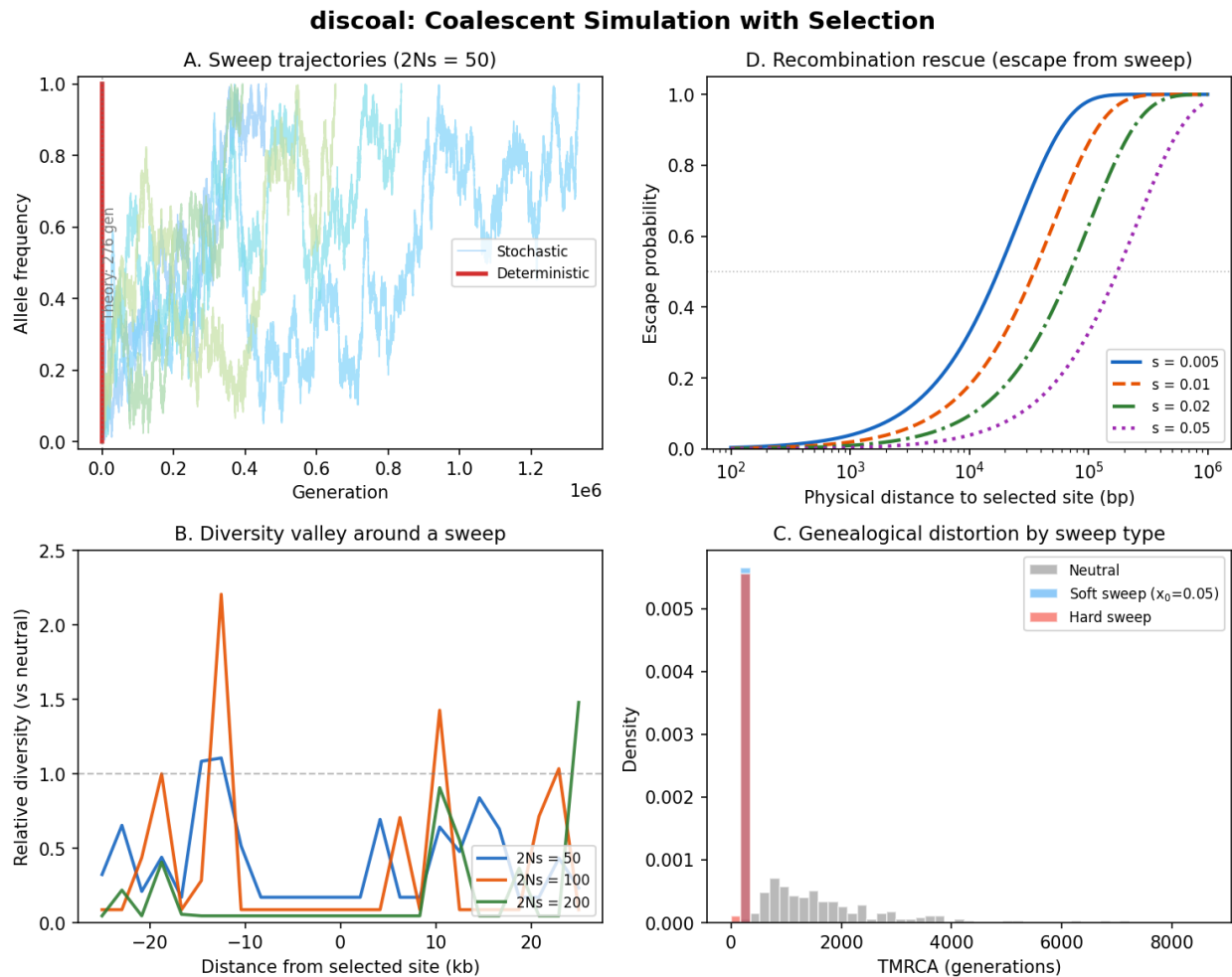
Fig. 35: discoal at a glance. Selective sweep signatures produced by the structured coalescent under selection. Panel A: Deterministic (logistic) vs stochastic allele frequency trajectories for a beneficial mutation sweeping to fixation. Panel B: The diversity valley – relative diversity drops near the selected site, with stronger selection producing deeper and narrower valleys. Panel C: Genealogical distortion by sweep type – hard sweeps compress TMRCA far more than soft sweeps. Panel D: Escape probability – the chance a neutral lineage recombines free of the sweep, as a function of physical distance from the selected site.
