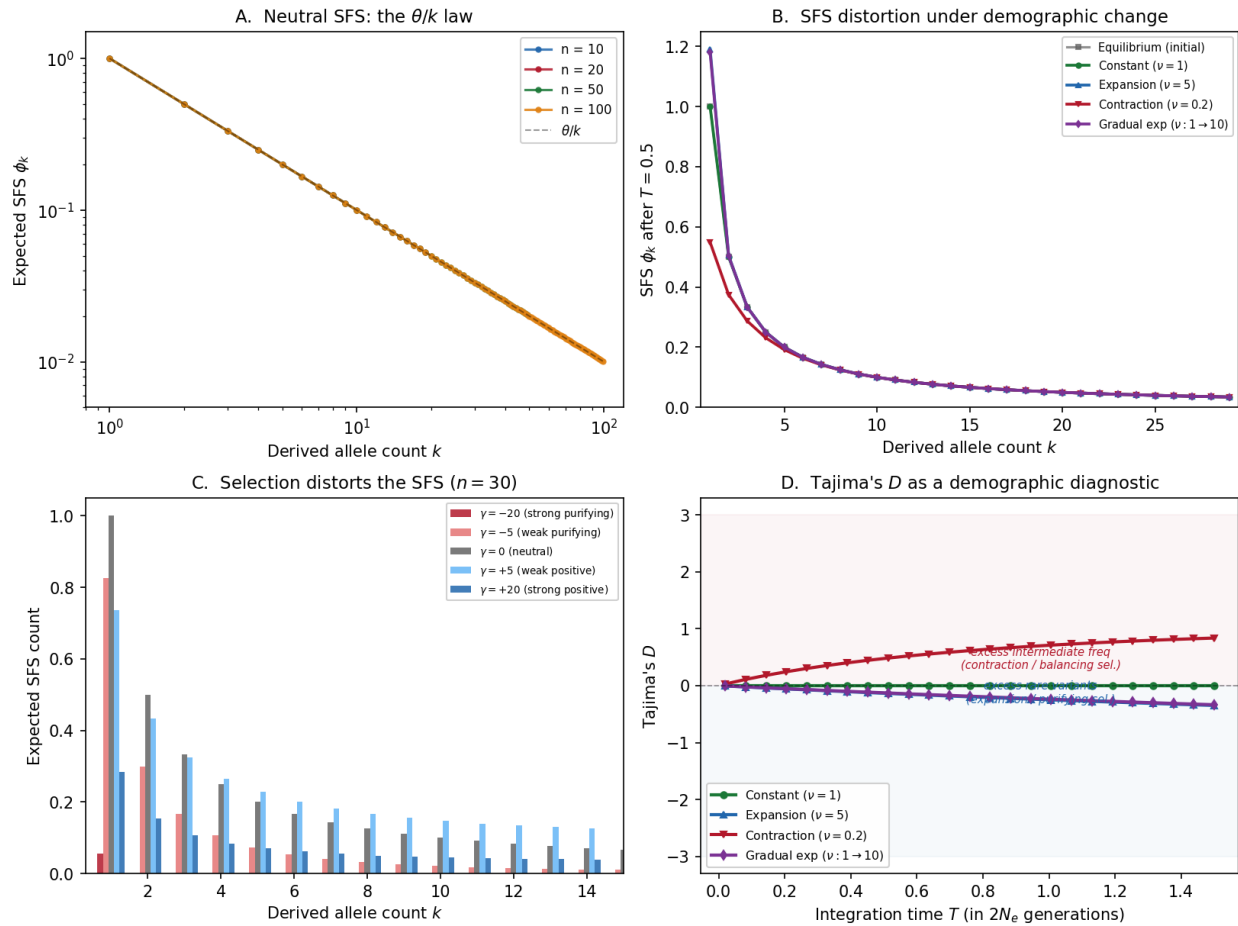
Fig. 19: moments at a glance . Panel A: The neutral site frequency spectrum for different sample sizes, showing the classic \theta/k pattern. Panel B: SFS evolution under drift – how the neutral spectrum deforms under population expansion vs contraction. Panel C: Selection’s effect on the SFS – positive selection shifts mass toward high frequencies, negative selection toward low frequencies. Panel D: Tajima’s D under expansion, constant size, and contraction, illustrating how summary statistics capture demographic signals.
