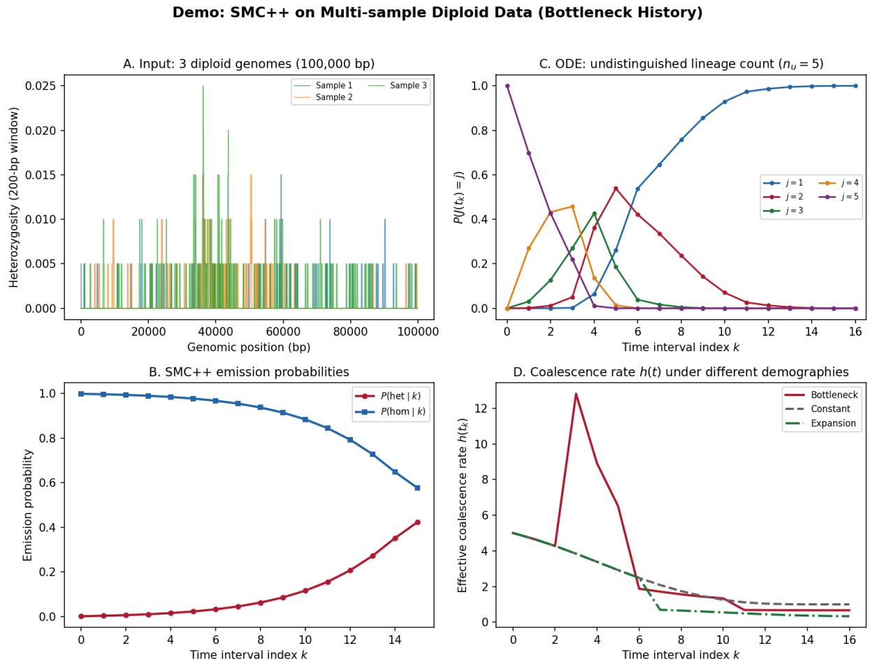
Fig. 4: SMC++ demo on msprime-simulated data. Panel A: Input heterozygosity tracks from multiple diploid genomes simulated under a bottleneck history. Panel B: SMC++ emission probabilities for het/hom observations at different coalescence times – P(\text{het} | k) rises with coalescence time as mutation accumulates. Panel C: ODE solution for undistinguished lineage probabilities P(J(t)=j) across time intervals under the bottleneck demography. Panel D: Effective coalescence rate h(t) under bottleneck, constant, and expansion demographic histories.
