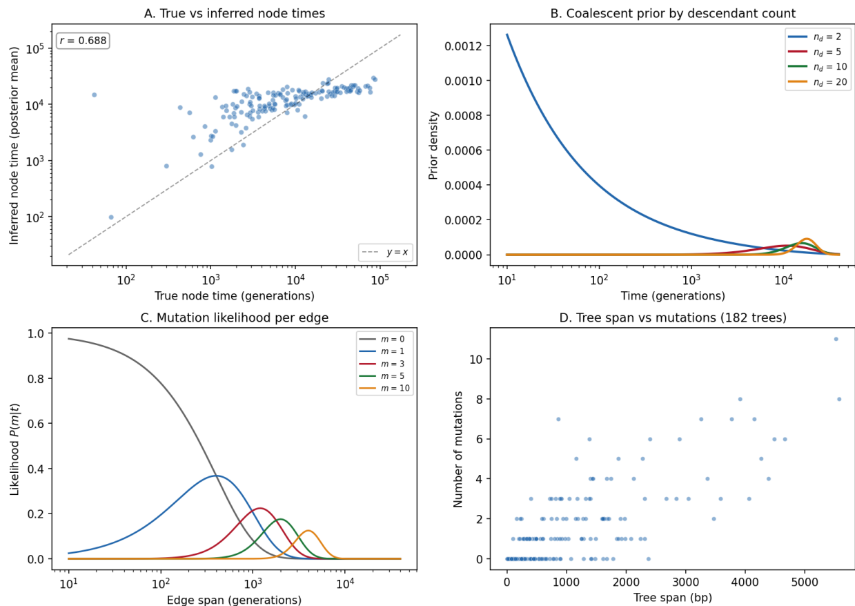
Fig. 18: tsdate demo on msprime -simulated data. Panel A: True vs inferred node times – gamma posterior means compared to true coalescence times. Panel B: Coalescent prior distributions by descendant count. Panel C: Mutation likelihood functions for different mutation counts. Panel D: Tree span vs number of mutations across the tree sequence.
