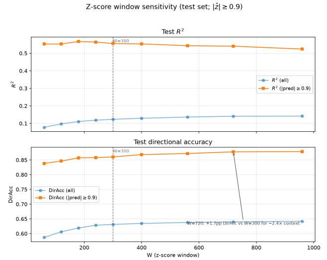
Figure 3: Z-score window w vs test R^2 and directional accuracy under |\hat{z}| \geq 0.9 . Past w=300 , additional lookback mainly increases required context while DirAcc gains flatten.
