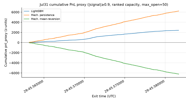
Figure 2: Cumulative z-unit proxy P&L over the Jul 31 session at \tau=0.9 (ranked capacity). This is a proxy in z-score units gross of costs, not a currency return; see Section 7.1.
