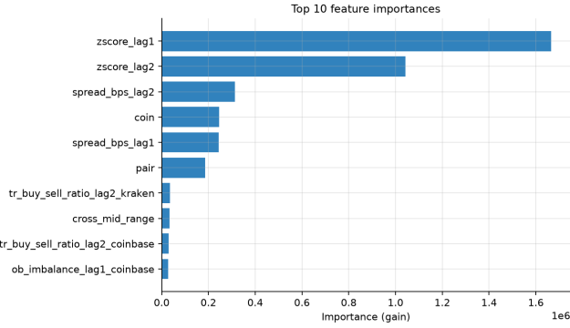
Figure 3: Top 10 features by LightGBM split gain. Gain is overwhelmingly concentrated in lagged z-scores and spread terms; microstructure features appear only in the lower ranks.
