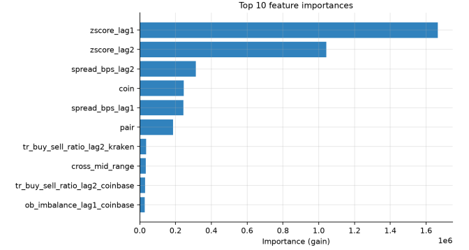
Figure 4: Top 10 features by LightGBM split gain. Gain is overwhelmingly concentrated in lagged z-scores and spread terms; microstructure features appear only in the lower ranks.
