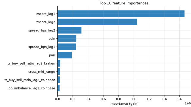
Figure 5: Top 10 features by LightGBM split gain. Gain is overwhelmingly concentrated in lagged z-scores and spread terms; microstructure features appear only in the lower ranks.
