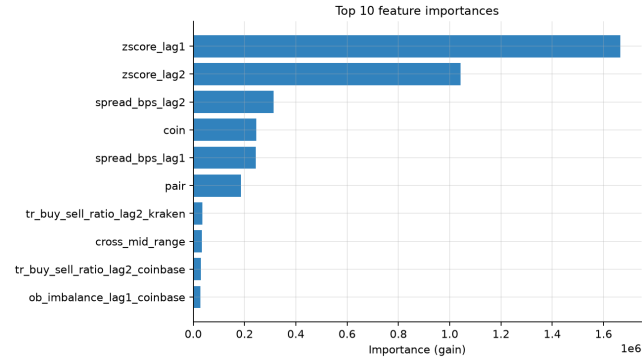
Figure 4: Top 10 features by LightGBM split gain. Gain is overwhelmingly concentrated in lagged z-scores and spread terms; rawer microstructure features appear only in the lower ranks.
