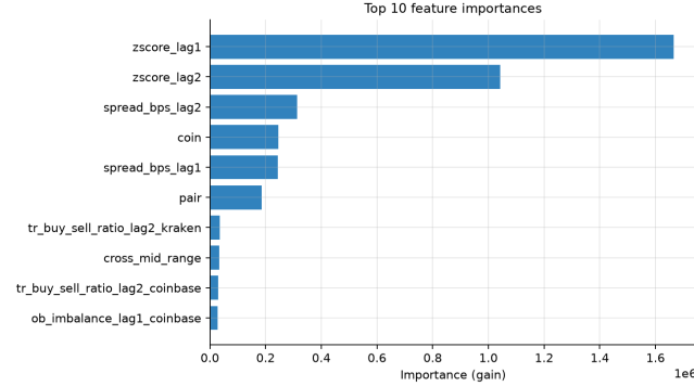
Figure 5: Top 10 features by LightGBM split gain.
