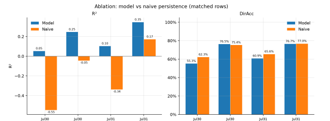
Figure 1: Model vs naive R^2 and directional accuracy across campaigns and filter conditions. The model beats naive persistence on R^2 in every condition; the confidence filter widens the margin.
